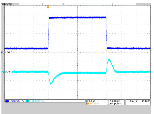
图 9-22. Load Transient Response
