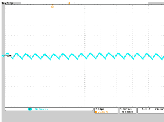
图 9-46. Output Voltage Ripple
