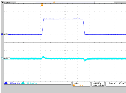
图 9-34. Line Transient Response
