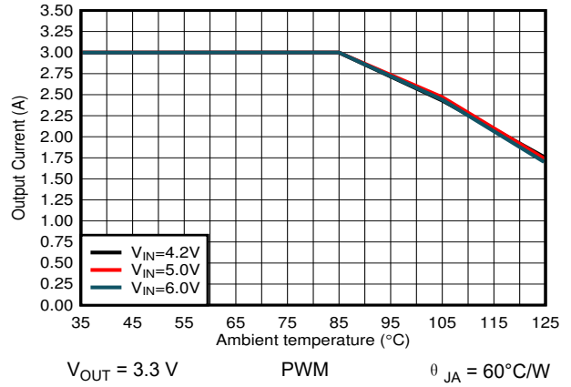
图 9-21. Output Current Versus Ambient Temperature
