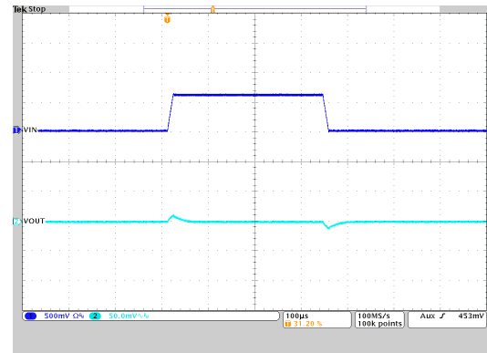
图 9-39. Line Transient Response
