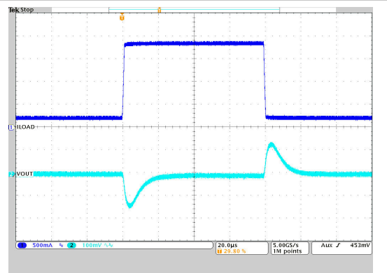
图 9-23. Load Transient Response
