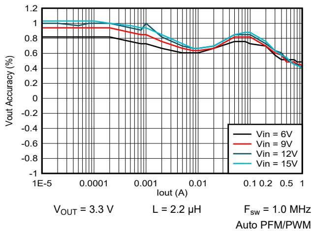
图 9-62. Output Voltage vs Output Current
