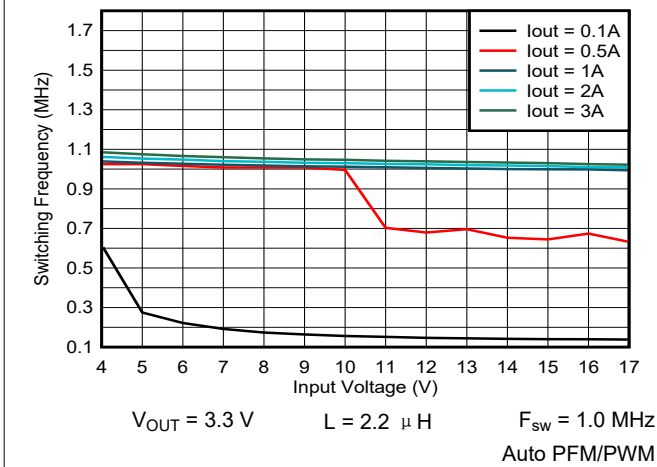
图 9-60. Switching Frequency vs Input Voltage
