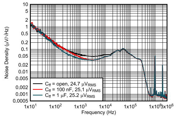
图 6-32. Output Noise Density vs Frequency
