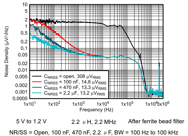
图 6-42. Output Noise Density vs Frequency
