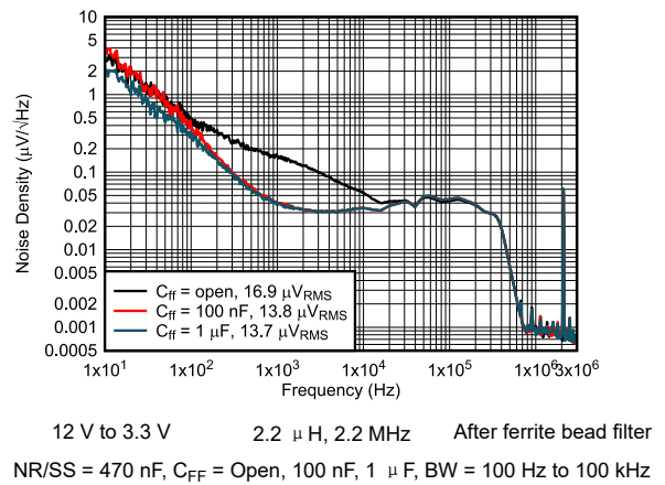
图 6-40. Output Noise Density vs Frequency
