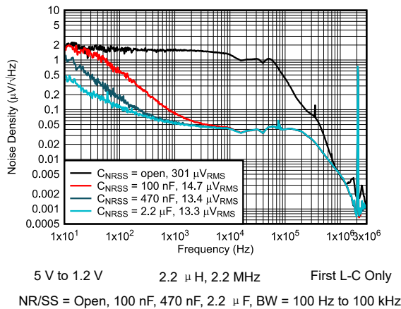
图 6-41. Output Noise Density vs Frequency
