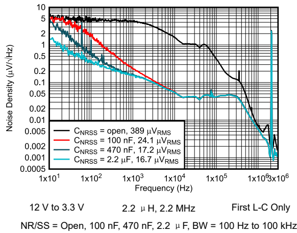
图 6-37. Output Noise Density vs Frequency
