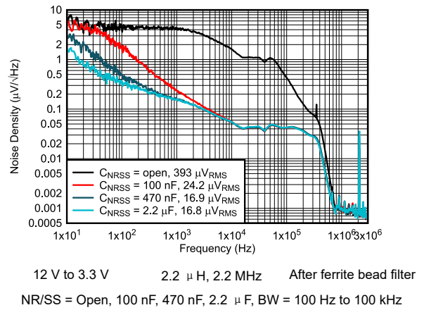
图 6-38. Output Noise Density vs Frequency
