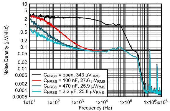
图 6-32. Output Noise Density vs Frequency
