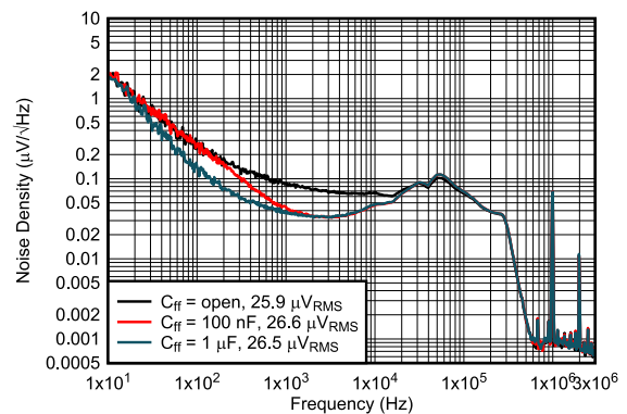
图 6-34. Output Noise Density vs Frequency
