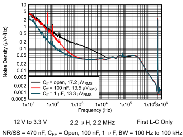
图 6-39. Output Noise Density vs Frequency
