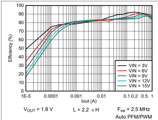
图 9-26. Efficiency vs Output Current
