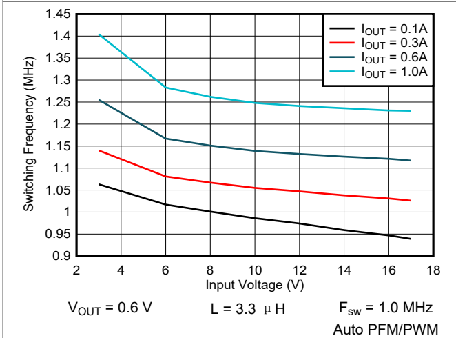
图 9-58. Switching Frequency vs Input Voltage
