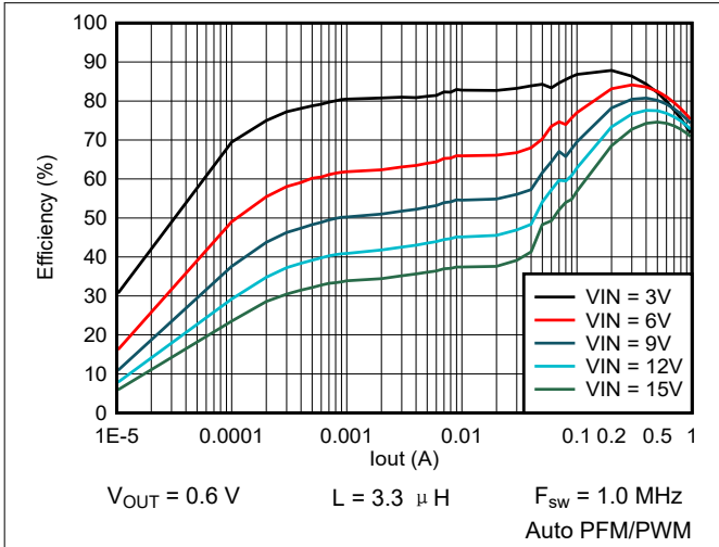
图 9-56. Efficiency vs Output Current
