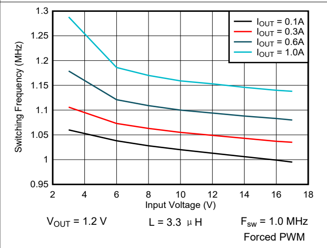
图 9-47. Switching Frequency vs Input Voltage
