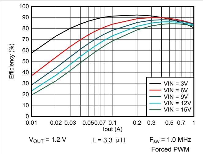
图 9-45. Efficiency vs Output Current
