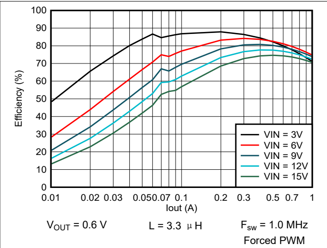
图 9-57. Efficiency vs Output Current
