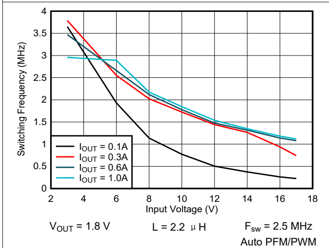
图 9-28. Switching Frequency vs Input Voltage
