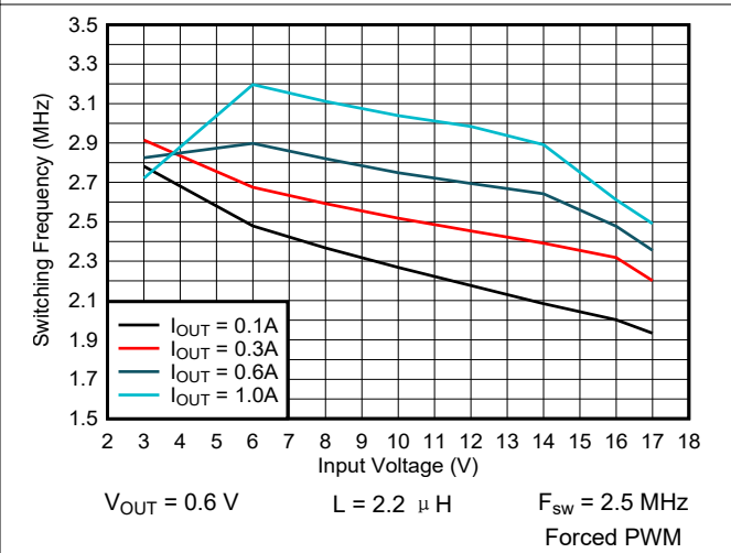
图 9-53. Switching Frequency vs Input Voltage
