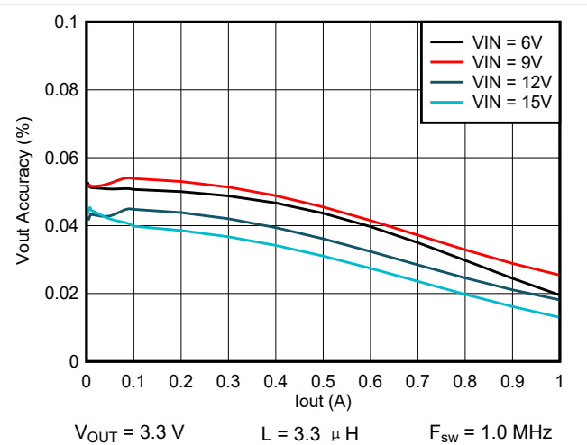
图 9-25. Output Voltage vs Output Current
