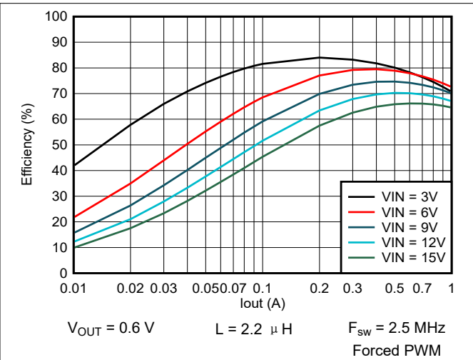
图 9-51. Efficiency vs Output Current
