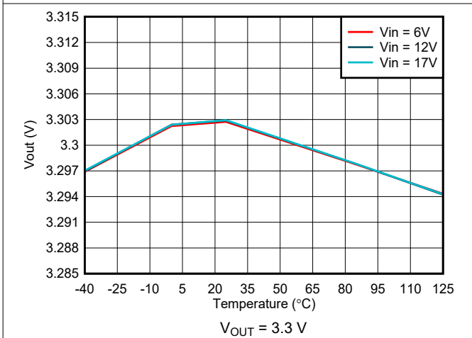
图 7-5. Output Voltage Accuracy - VSET Selected
