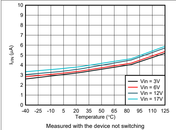
图 7-1. Typical Quiescent Current vs Temperature
