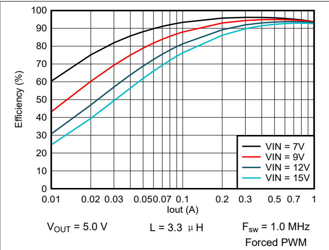
图 9-9. Efficiency vs Output Current
