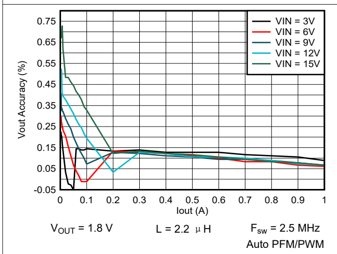
图 9-30. Output Voltage vs Output Current
