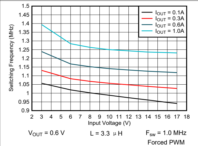
图 9-59. Switching Frequency vs Input Voltage
