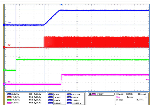
图 9-63. Start-Up Timing
