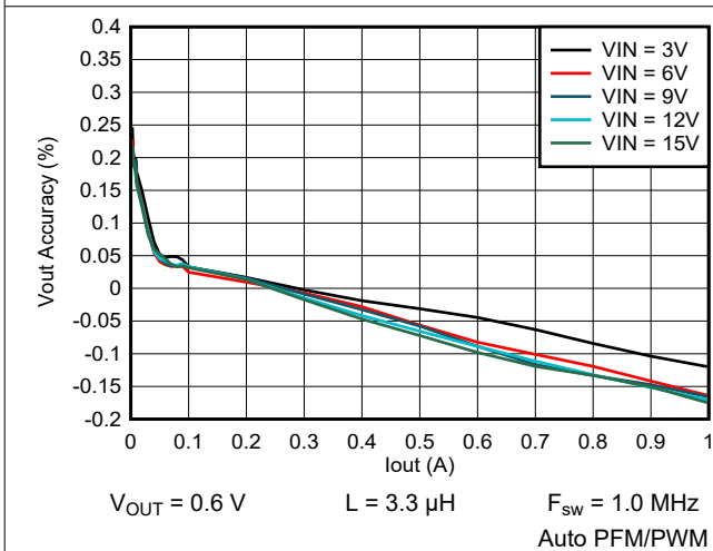
图 9-60. Output Voltage vs Output Current
