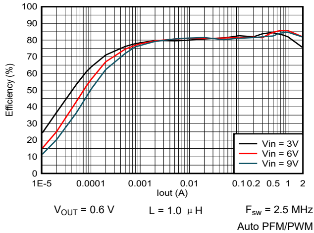
图 9-27. Efficiency vs Output Current
