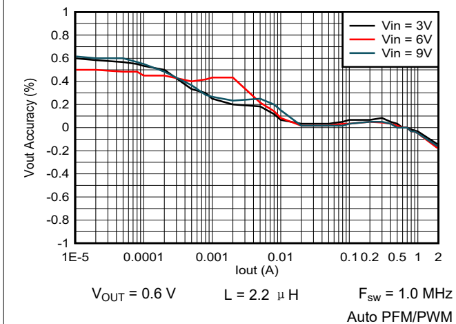
图 9-37. Output Voltage vs Output Current
