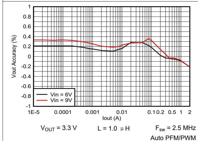
图 9-56. Output Voltage vs Output Current
