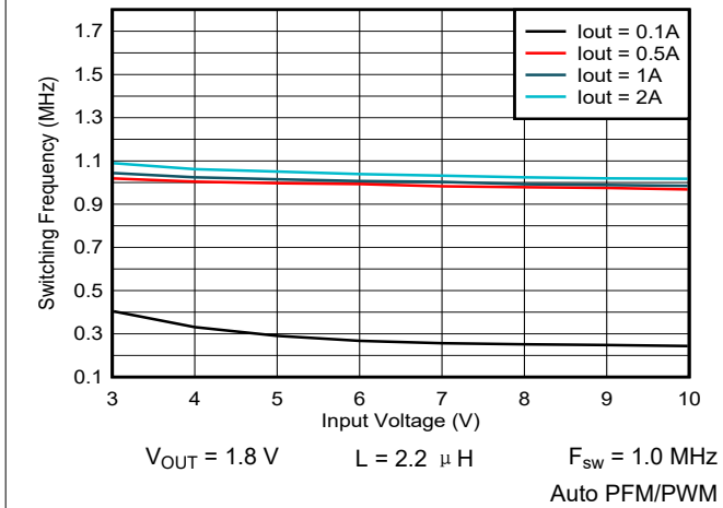
图 9-11. Switching Frequency vs Input Voltage
