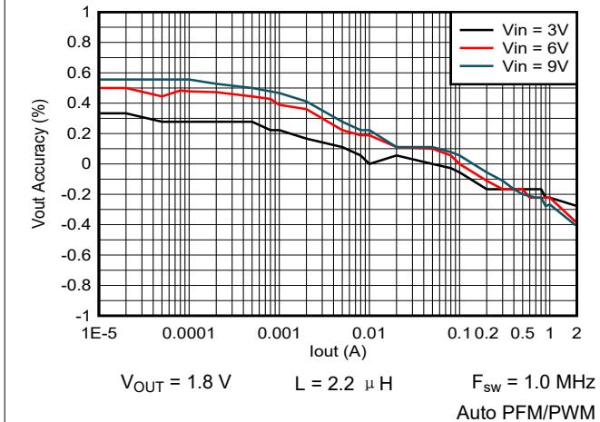
图 9-13. Output Voltage vs Output Current
