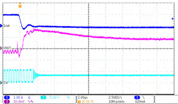
图 9-72. Load Transient Response
