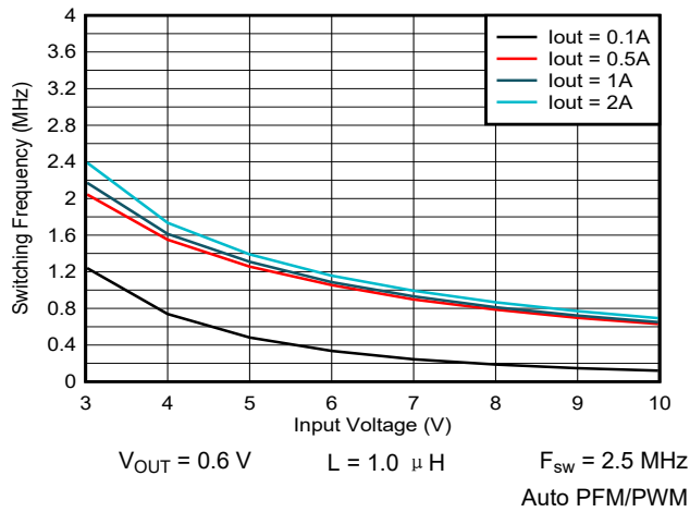
图 9-29. Switching Frequency vs Input Voltage
