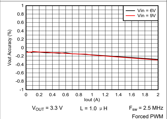
图 9-57. Output Voltage vs Output Current
