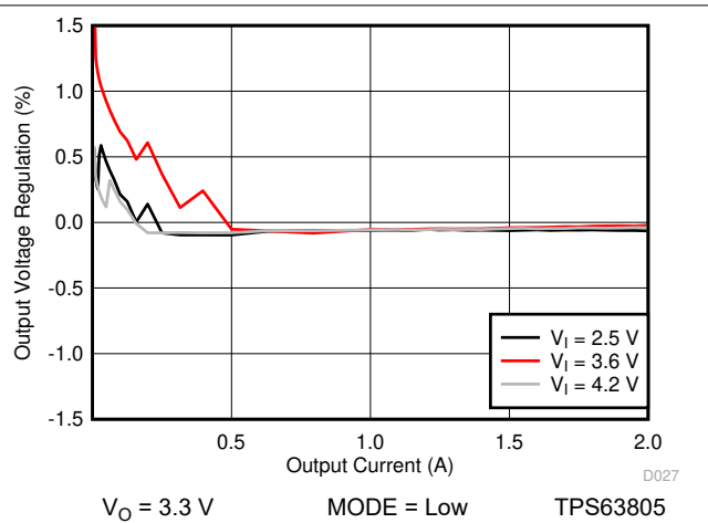
图 10-20. Load Regulation (PFM/PWM)
