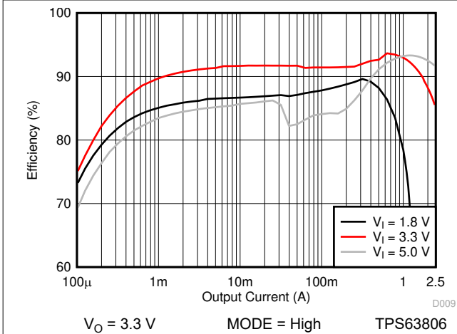
图 10-15. Efficiency versus Output Current (PFM/PWM)
