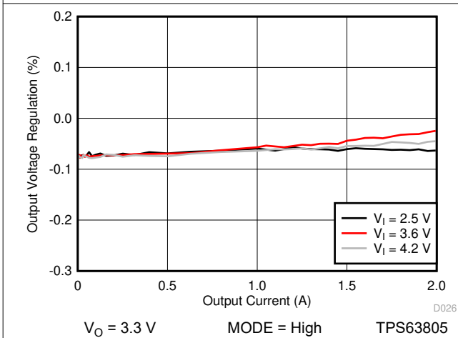
图 10-19. Load Regulation (PWM Only)
