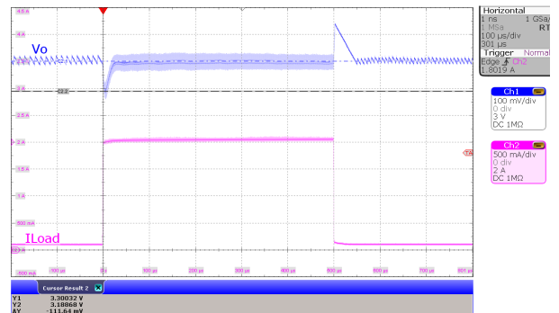
V_I = 2.8\text{ V} , V_O = 3.3\text{ V} I_O from 100 mA to 2 A t_r = 1\ \mu\text{s} , t_f = 1\ \mu\text{s} TPS63806 MODE = Low
