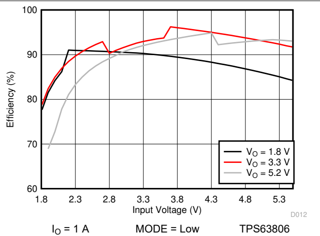
图 10-18. Efficiency versus Input Voltage (PWM Only)
