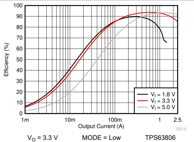
图 10-16. Efficiency versus Input Voltage (PWM Only)
