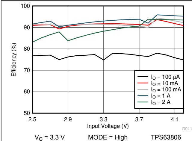
图 10-17. Efficiency versus Input Voltage (PFM/PWM)
