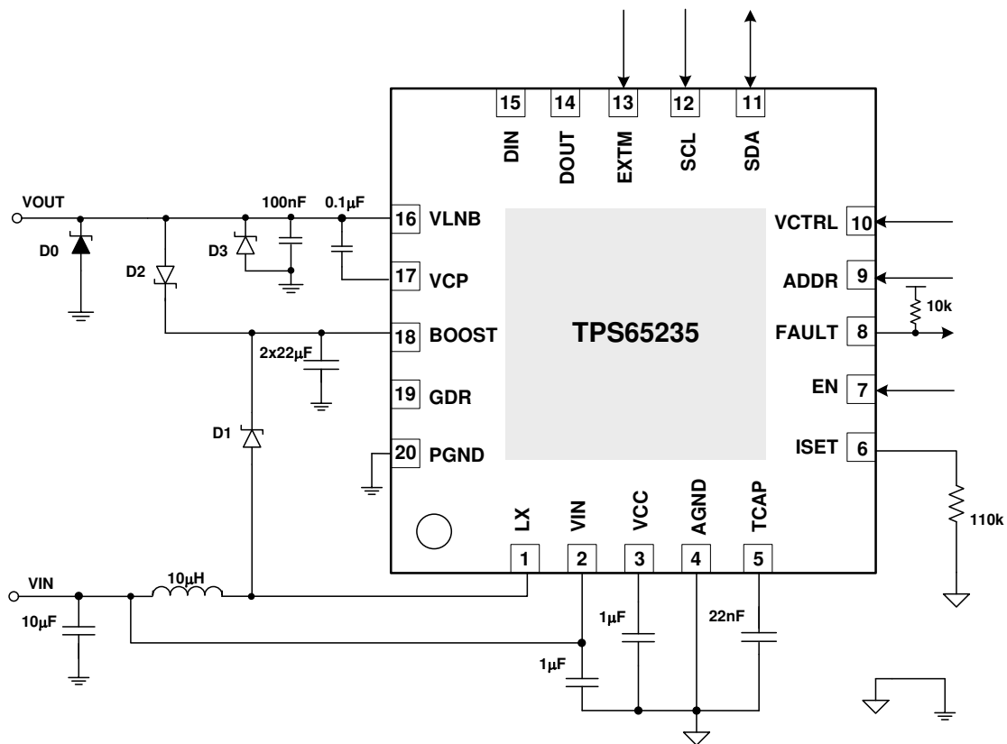
图 8-1. Application for DiSEqC1.x Support
