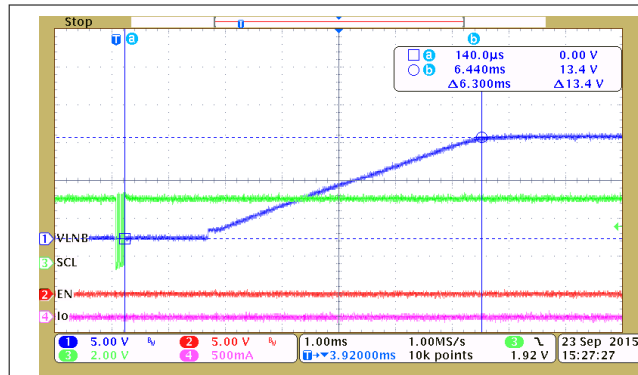
图 7-3. VLNB Output Controlled by bit EN of Control Register 2
