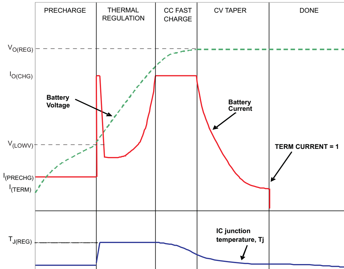
Figure 12. Thermal Loop
