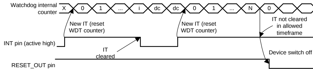
图 5-24. Watchdog Timings—Interrupt Mode
