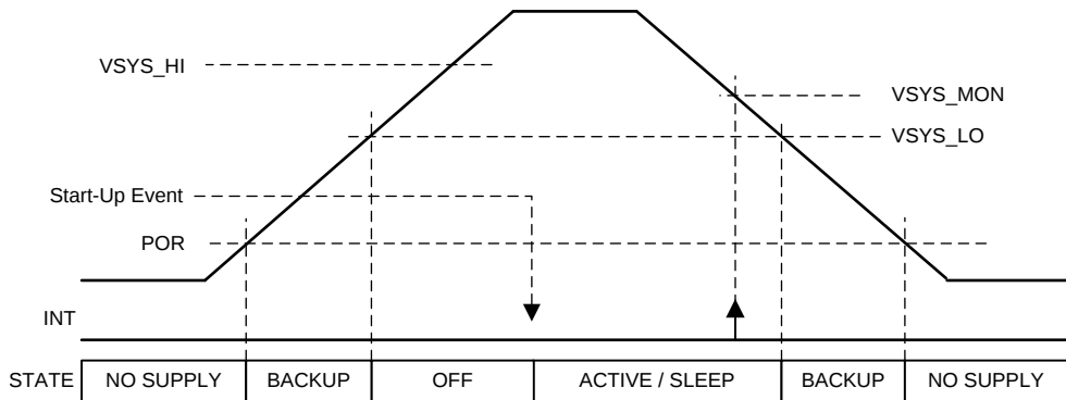
图 5-26. State Transitions
