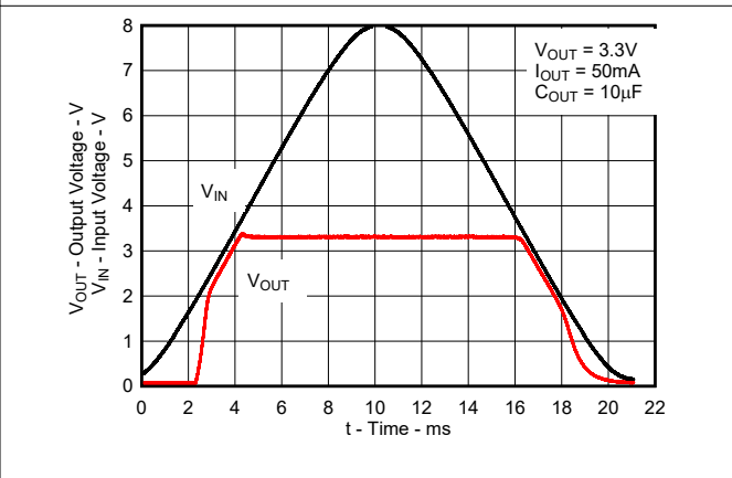
图 5-24. TPS71433 Power-Up, Power-Down (New Chip)
