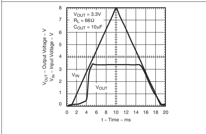
图 5-23. TPS71433 Power-Up, Power-Down (Legacy Chip)
