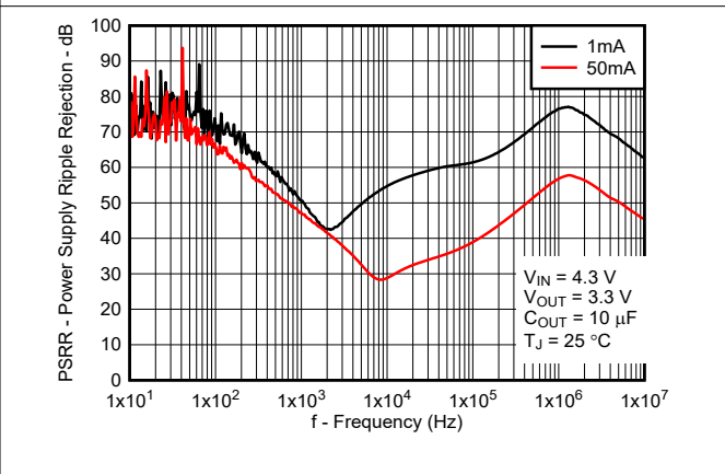
图 5-22. TPS71433 Power-Supply Ripple Rejection vs Frequency (New Chip)
