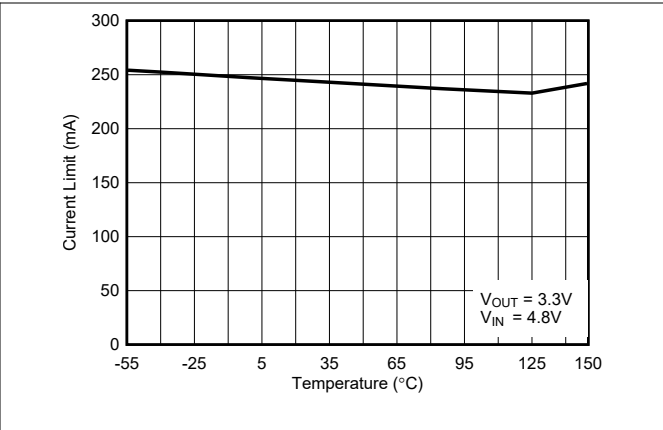
图 5-20. TPS71433 Current Limit vs Junction Temperature (New Chip)
