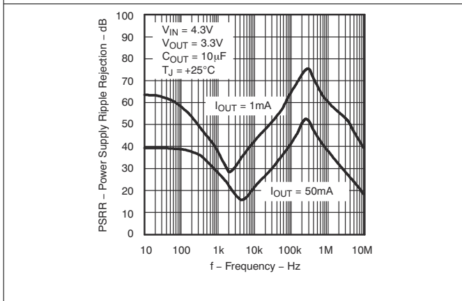
图 5-21. TPS71433 Power-Supply Ripple Rejection vs Frequency (Legacy Chip)
