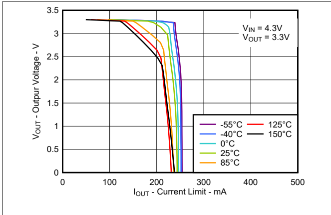
图 5-19. TPS71433 V_{OUT} vs Current Limit (New Chip)
