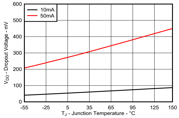
图 6-14. Dropout Voltage vs Free-Air Temperature for New Chip
