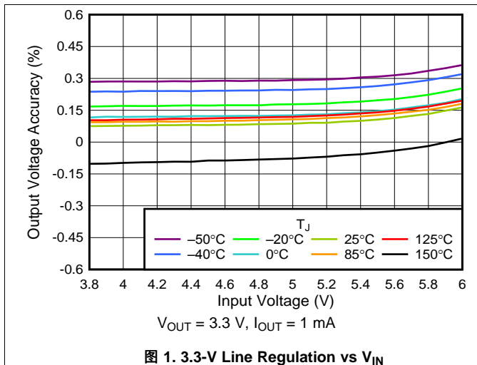
图 1. 3.3-V Line Regulation vs V_{IN}
