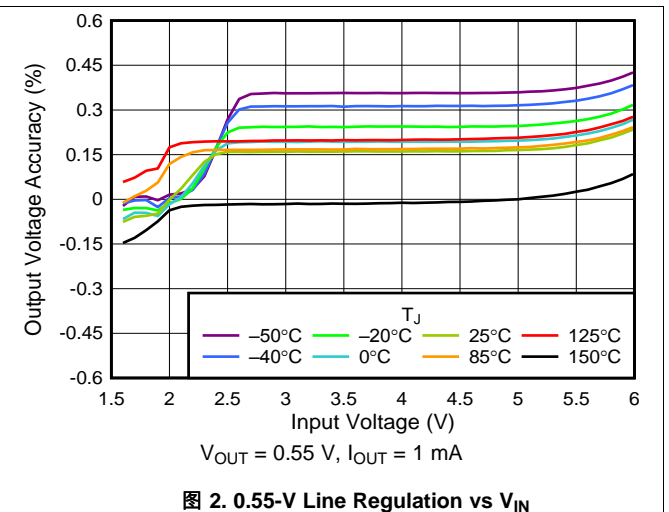
图 2. 0.55-V Line Regulation vs V_{IN}
