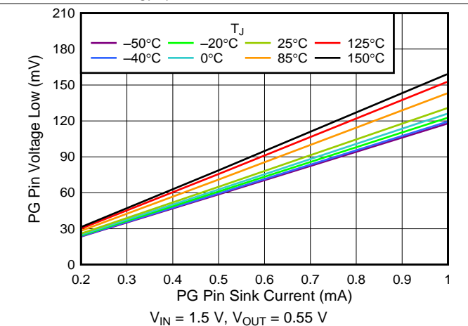
图 18. V OL (PG) vs PG Pin Sink Current
