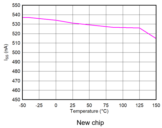
图 5-28. Soft-Start Charging Current (I SS ) vs Temperature (T J )
