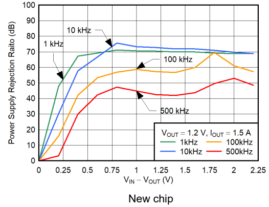
图 5-20. V IN PSRR vs (V IN - V OUT )
