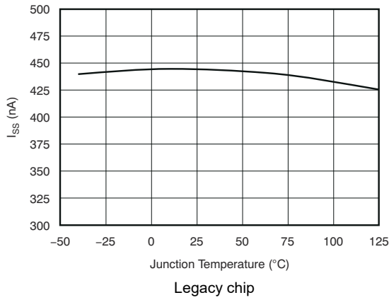
图 5-27. Soft-Start Charging Current (I SS ) vs Temperature (T J )
