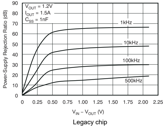
图 5-19. V IN PSRR vs (V IN - V OUT )
