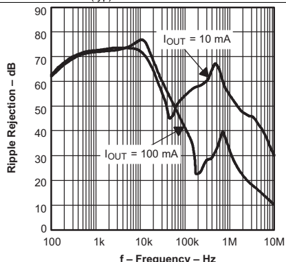
V_{IN} = 2.8\text{ V} , C_{OUT} = 1\text{ }\mu\text{F} , C_{BYPASS} = 0.01\text{ }\mu\text{F}
