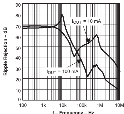
V_{IN} = 2.8\text{ V} , C_{OUT} = 1\text{ }\mu\text{F} , C_{BYPASS} = 0.1\text{ }\mu\text{F}
