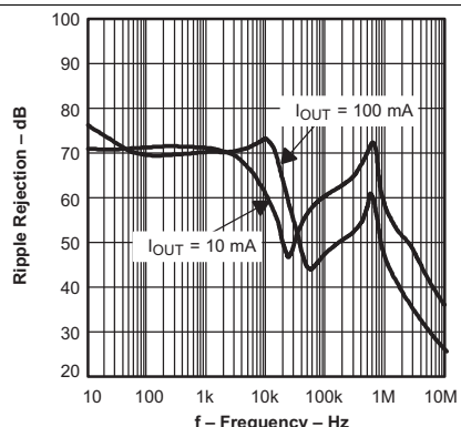
V_{IN} = 4.3\text{ V} , C_{OUT} = 10\text{ }\mu\text{F} , C_{BYPASS} = 0.01\text{ }\mu\text{F}
