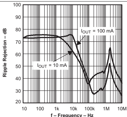
V_{IN} = 4.3\text{ V} , C_{OUT} = 1\text{ }\mu\text{F} , C_{BYPASS} = 0.1\text{ }\mu\text{F}
