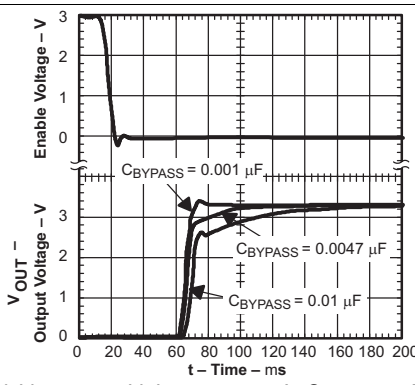
V_{IN} = 4.3\text{ V} , V_{OUT} = 3.3\text{ V} , I_{OUT} = 100\text{ mA} , C_{OUT} = 1\text{ }\mu\text{F} , T_J = 25^\circ\text{C}
