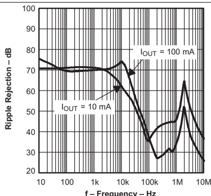
V_{IN} = 4.3\text{ V} , C_{OUT} = 1\text{ }\mu\text{F} , C_{BYPASS} = 0.01\text{ }\mu\text{F}
