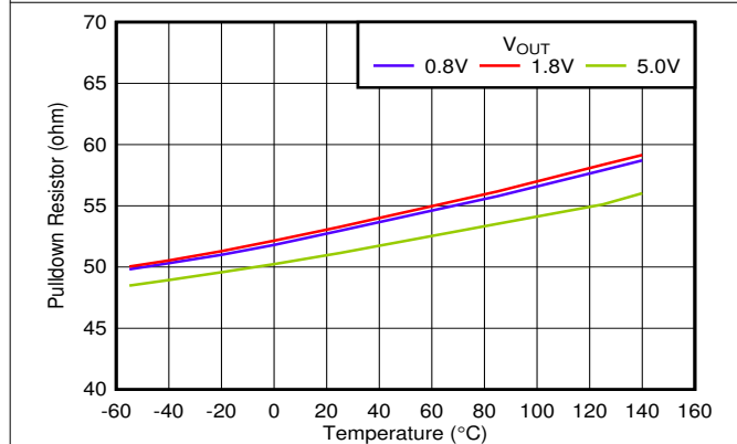
图 6-41. Pulldown Resistor vs Temperature and V_{OUT}
