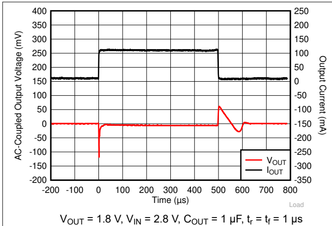
图 6-13. I_{OUT} Transient From 1 mA to 100 mA
