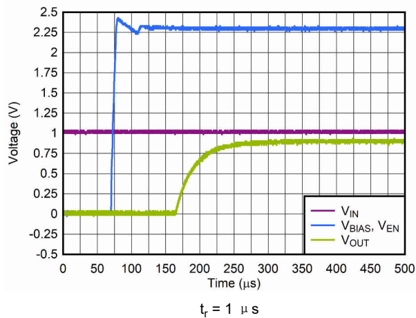
图 6-15. Start-Up With V_{IN} Before V_{BIAS} and V_{EN}
