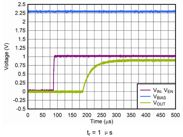
图 6-14. Start-Up With V_{BIAS} Before V_{IN}
