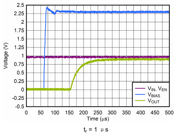
图 6-17. Start-Up With V_{IN} and V_{EN} Before V_{BIAS}
