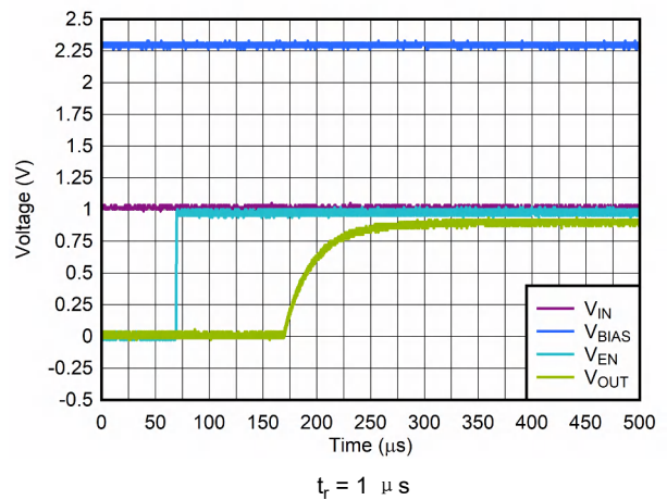
图 6-16. Start-Up With V_{IN} and V_{BIAS} Before V_{EN}
