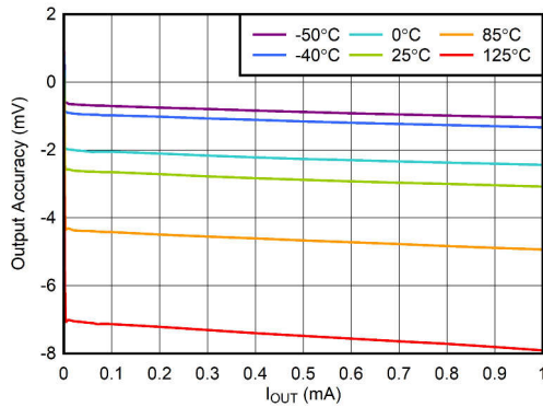
图 6-3. Output Voltage Accuracy vs I_{OUT}
