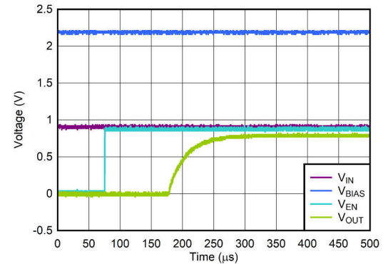
图 6-14. Start-Up With V_{\text{BIAS}} Before V_{\text{IN}}
