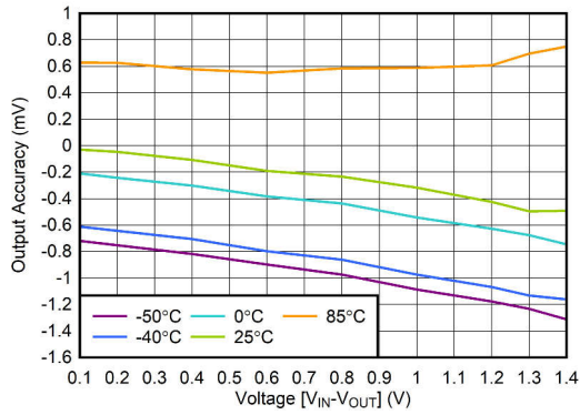
图 6-1. Output Voltage Accuracy vs V_{IN}
