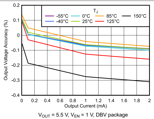
图 5-20. Output Voltage Accuracy vs I_{OUT}
