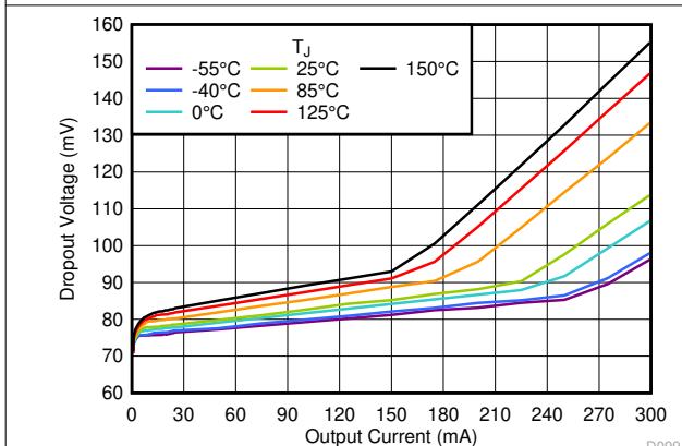
图 5-27. Dropout Voltage vs I_{OUT}
