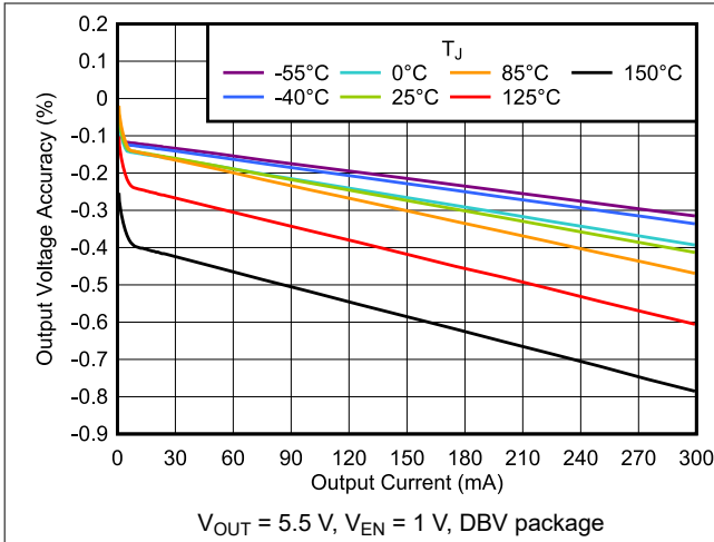
图 5-19. Output Voltage Accuracy vs I_{OUT}
