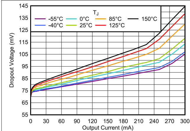
图 5-25. Dropout Voltage vs I_{OUT}
