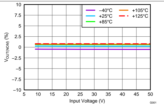
Figure 2. Line Regulation
