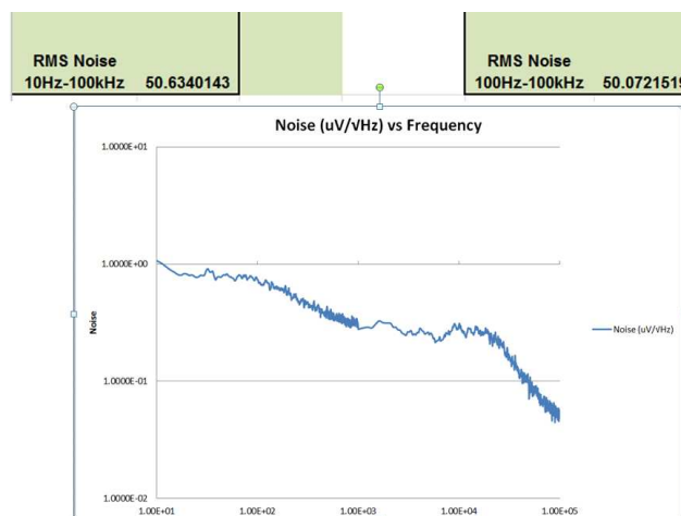
Figure 26. Output Noise Plot, V_{IN} = 7\text{ V} , V_{OUT} = 5\text{ V} at 750 mA, C_{OUT} = 22\text{ }\mu\text{F} Tantalum Capacitor
