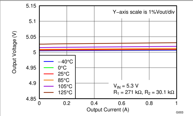
图 5-2. Load Regulation (5 V, Adjustable)
