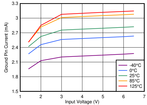
V_{BIAS} = 0\text{ V} , I_{OUT} = 5\text{ mA} 图 6-32. Ground Pin Current vs V_{IN}
