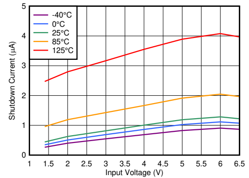
V_{BIAS} = 0\text{ V} 图 6-34. Shutdown Current vs V_{IN}
