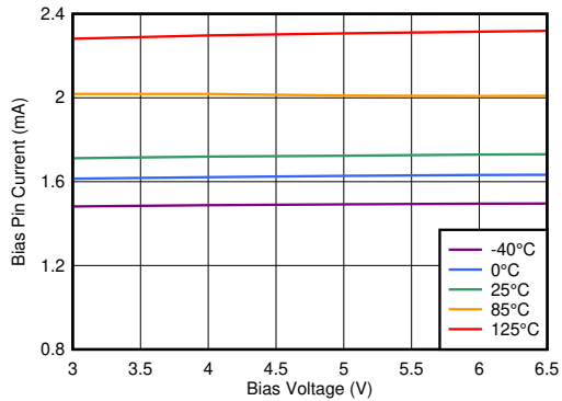
V_{IN} = 1.1\text{ V} , I_{OUT} = 5\text{ mA} 图 6-33. Bias Pin Current vs Bias Voltage
