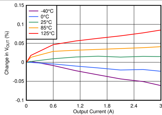
图 6-26. Load Regulation vs I_{OUT}
