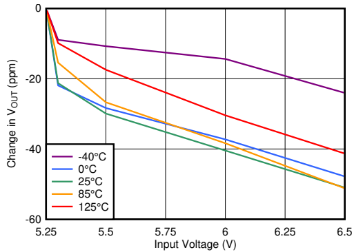
I_{OUT} = 5\text{ mA} 图 6-31. Line Regulation vs V_{IN} (5-V Output)
