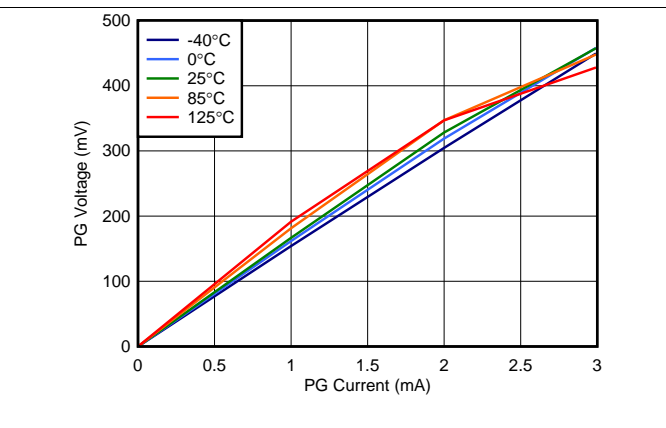
图 34. PGx Low Level vs PGx Current ( V_{\text{INX}} = 1.4\text{ V} )
