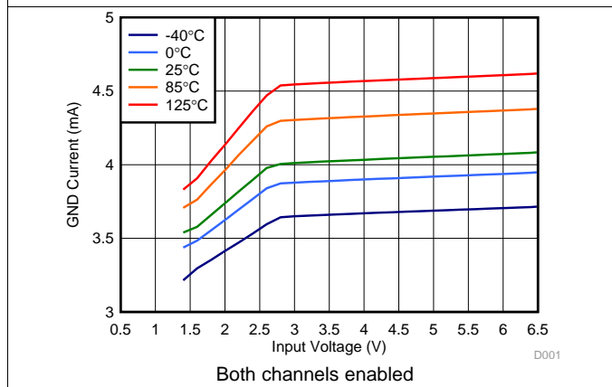
图 33. Ground Current vs Input Voltage
