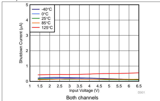
图 31. Shutdown Current vs Input Voltage
