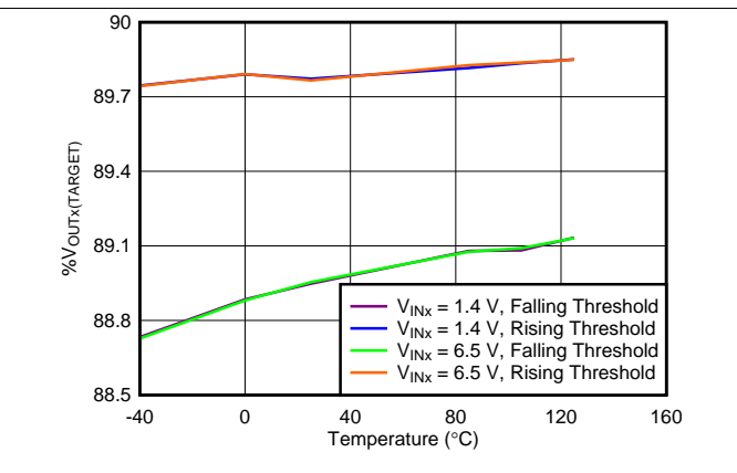
图 36. PGx Threshold vs Temperature
