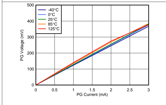
图 35. PGx Low Level vs PGx Current ( V_{\text{INX}} = 6.5\text{ V} )
