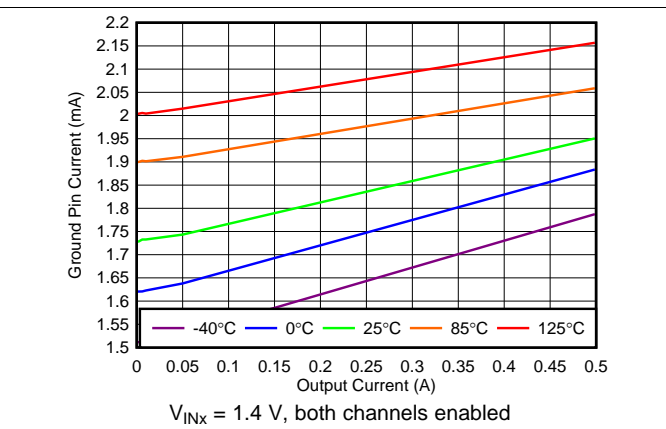
图 32. Ground Current vs Output Current
