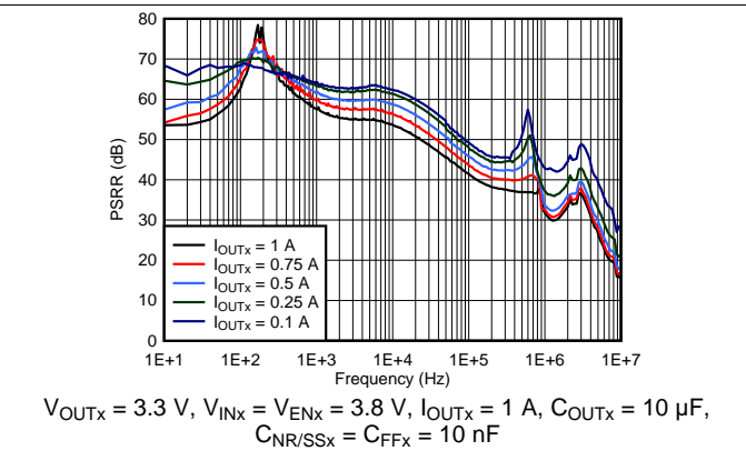
图 4. Power-Supply Rejection vs Output Current
