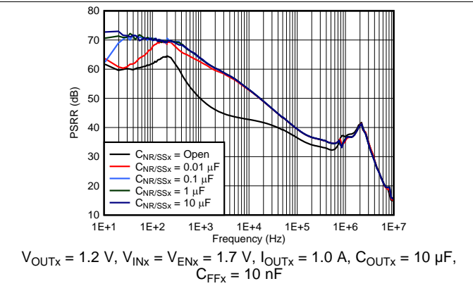
图 2. Power-Supply Rejection vs C_{NR/SSx}
