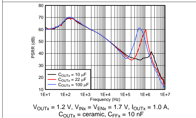
图 5. Power-Supply Rejection vs Output Capacitance
