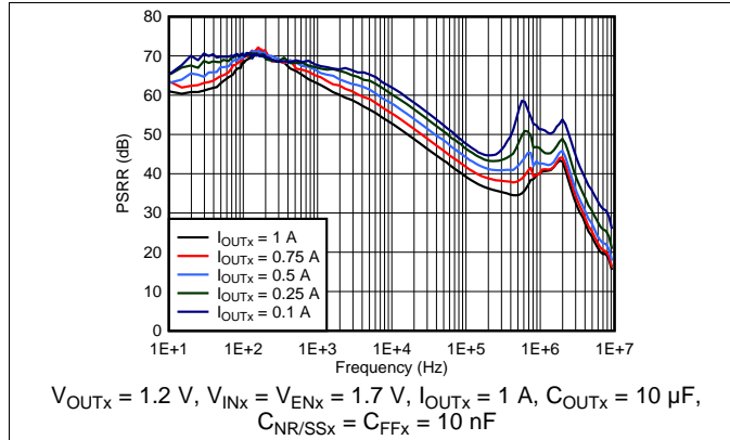
图 1. Power-Supply Rejection vs Output Current
