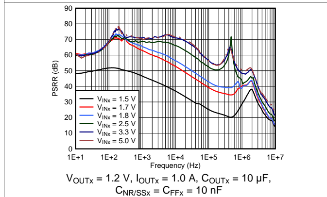
图 3. Power-Supply Rejection vs Input Voltage
