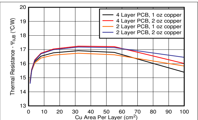
图 8-3. \psi_{JB} vs Copper Area 2s2p DCY Package
