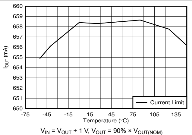
图 6-24. Output Current Limit vs Temperature
