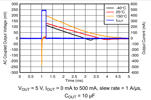
图 6-22. Load Transient, No Load to 500 mA
