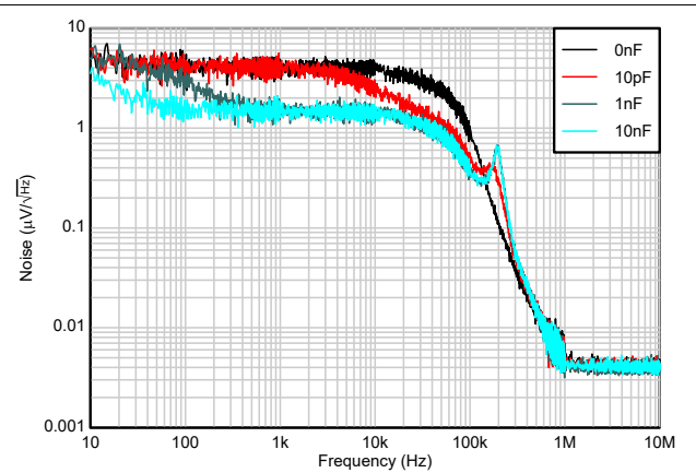
V_{IN} = 4.3\text{V} , V_{OUT} = 3.3\text{V} , C_{OUT} = 2.2\mu\text{F} , I_{OUT} = 150\text{mA}
