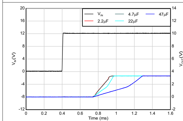
V_{IN} = 12\text{V} , V_{OUT} = 3.3\text{V} , I_{OUT} = 1\text{mA}
