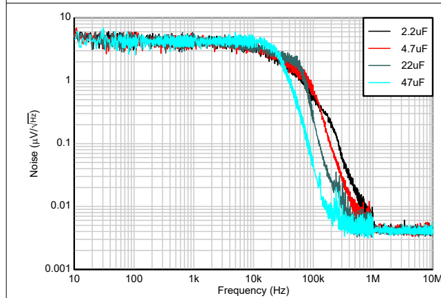
V_{IN} = 5.3\text{V} , V_{OUT} = 3.3\text{V} , I_{OUT} = 300\text{mA}
