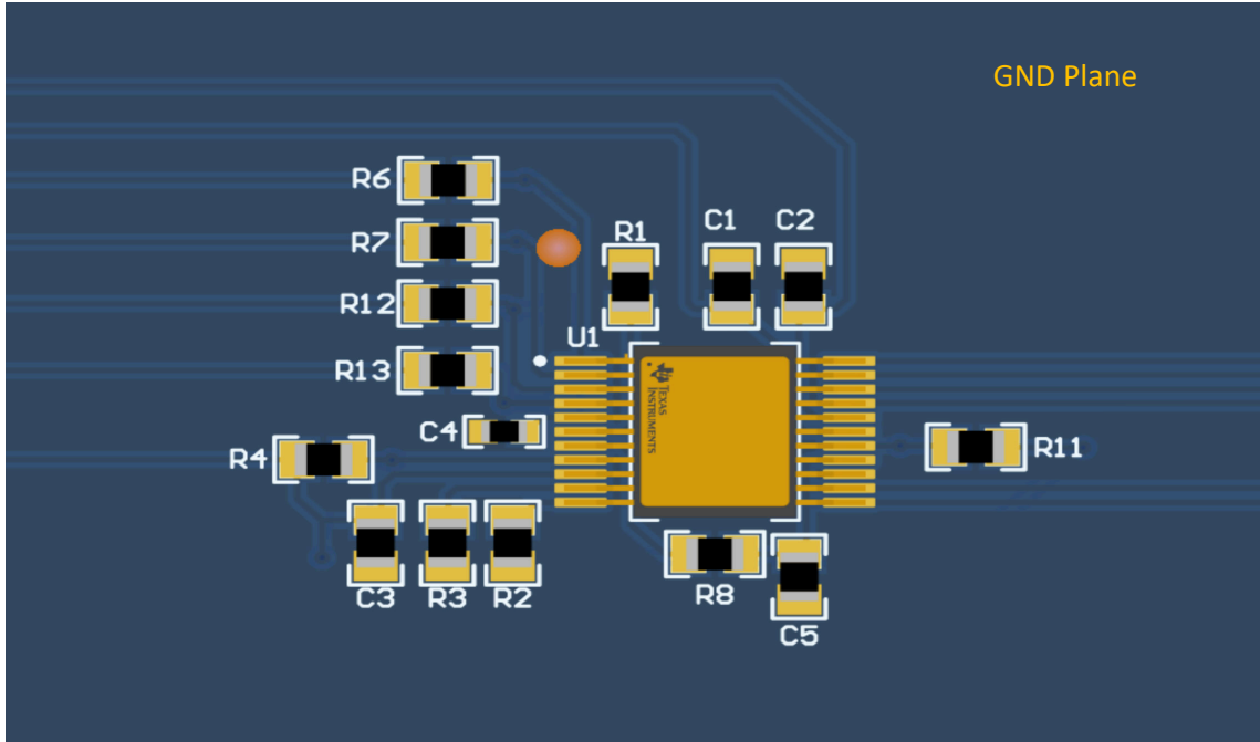
图 9-17. Printed Circuit Board Layout Example: Top Layer 3D View
