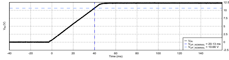
图 9-2. V_{IN} vs Time During Sequence UP
