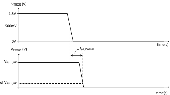
图 7-7. PWRGD Propagation Delay ( t_{pd\_PWRGD} ) Time Measurement - Falling Voltage
