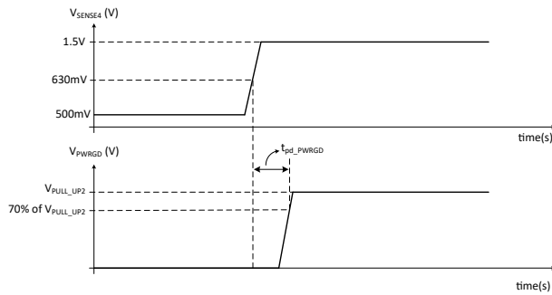
图 7-6. PWRGD Propagation Delay ( t_{pd\_PWRGD} ) Time Measurement - Rising Voltage
