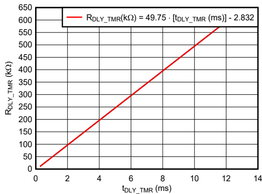
图 8-9. R_{DLY\_TMR} vs t_{DLY\_TMR} From 0.268ms to 12.5ms
