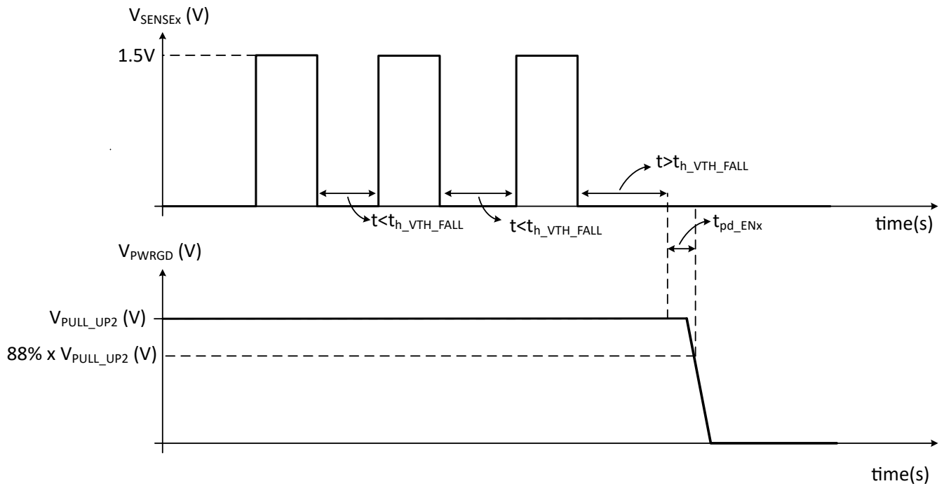
图 7-12. Falling Threshold on SENSEx Hold Time ( t_{h\_VTH\_FALL} )
