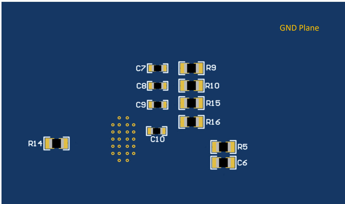
图 9-18. Printed Circuit Board Layout Example: Bottom Layer 3D View
