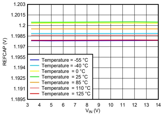
图 6-13. REFCAP vs V_{IN} Across Temperature
