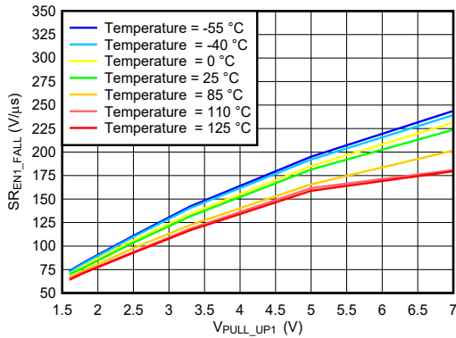
图 6-25. SR_{EN1\_FALL} vs V_{PULL\_UP1} Across Temperature
