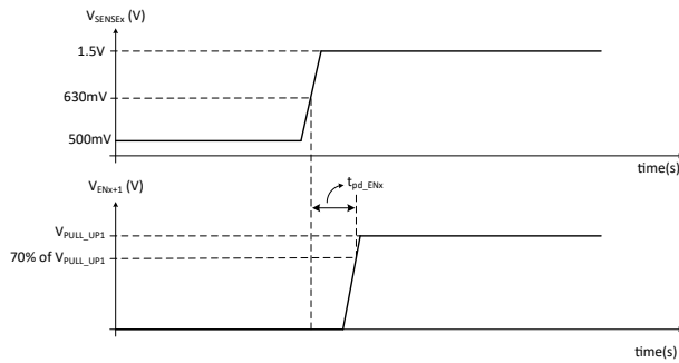
图 7-2. ENx Propagation Delay ( t_{pd\_ENx} ) Time Measurement - Rising Voltage
