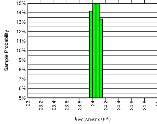
图 6-8. IHYS_SENSEx Current Distribution at Temperature of 25°C
