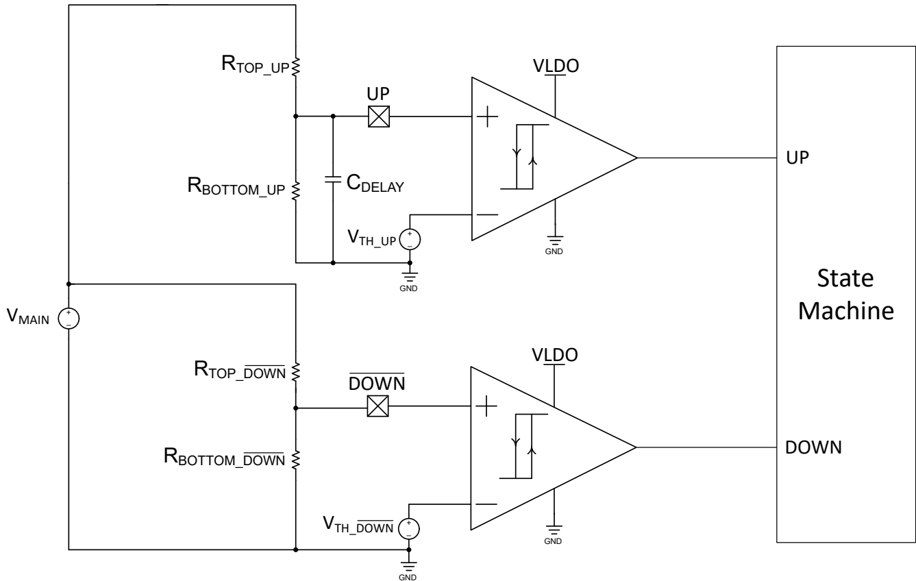
图 8-13. Monitor a Main Rail to Automatically Start the Sequence UP and \overline{DOWN}
