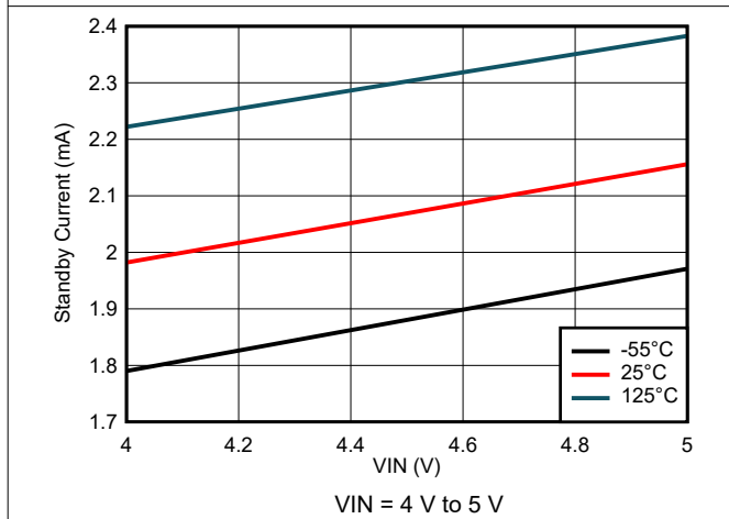
图 7-3. Standby Current Variation
