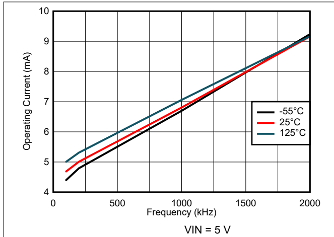
图 7-1. Operating Current Variation
