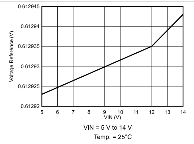
图 7-14. Voltage Reference Variation
