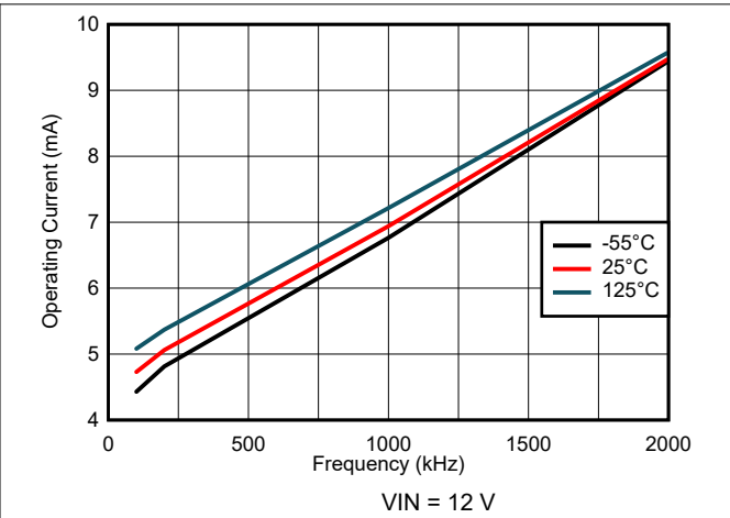
图 7-2. Operating Current Variation
