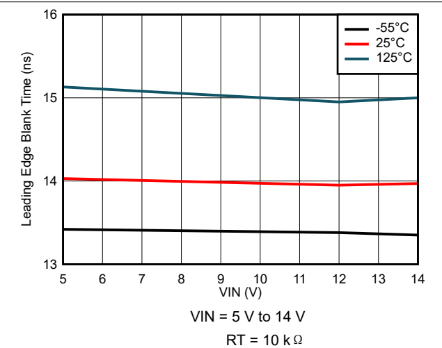
图 7-34. Leading Edge Blank Time Variation
