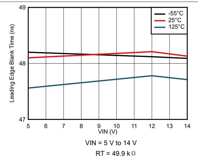
图 7-36. Leading Edge Blank Time Variation
