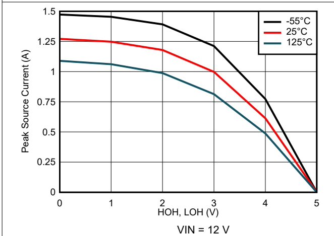
图 7-11. Peak Source Current vs Output Voltage
