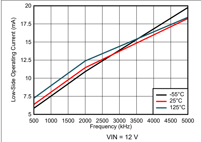
图 7-43. Low-Side Operating Current vs Frequency (PWM)
