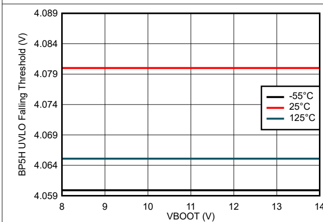
图 7-23. BP5H UVLO Falling Threshold vs BOOT Voltage
