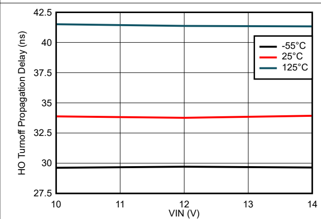
图 7-6. HO Turnoff Propagation Delay vs VIN Voltage (PWM)
