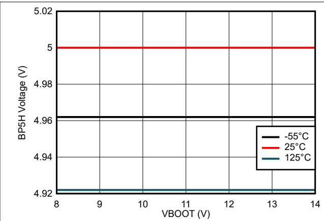
图 7-2. BP5H Output Voltage vs BOOT Voltage
