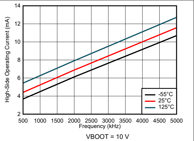
图 7-44. High-Side Operating Current vs Frequency (IIM)
