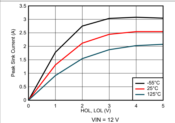
图 7-12. Peak Sink Current vs Output Voltage
