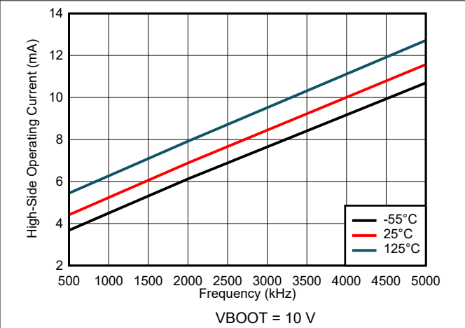
图 7-44. High-Side Operating Current vs Frequency (IIM)
