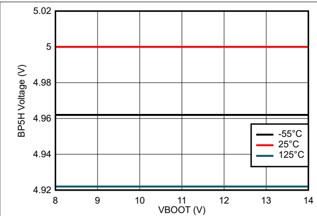
图 7-2. BP5H Output Voltage vs BOOT Voltage
