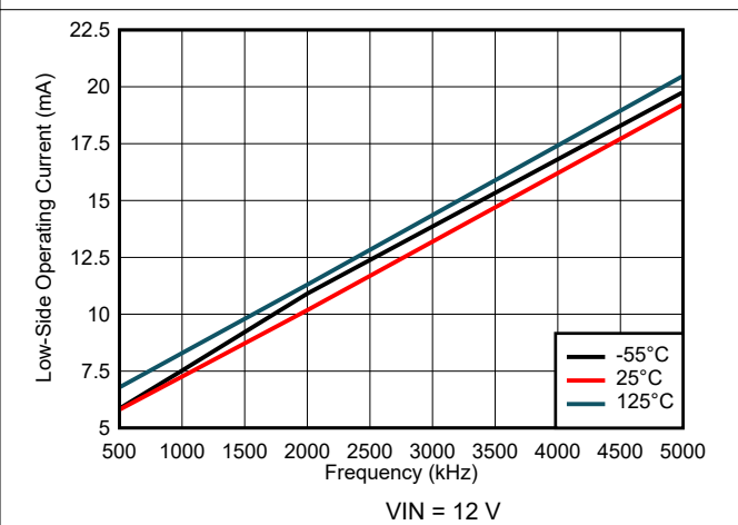
图 7-42. Low-Side Operating Current vs Frequency (IIM)
