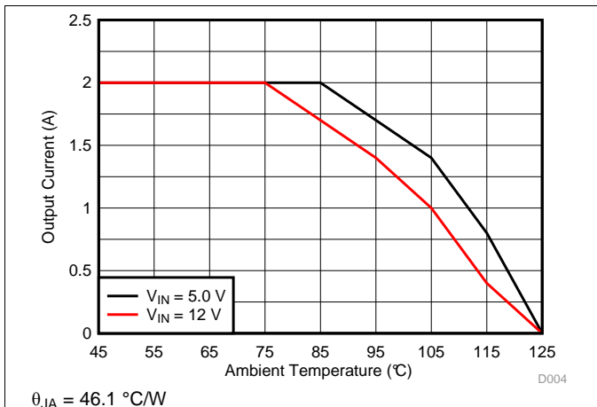
图 18. Thermal Derating, V_{OUT} = 3.3 \text{ V}
