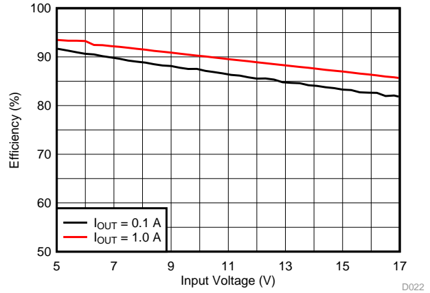
图 13. Efficiency, V_{OUT} = 3.3\text{ V}
