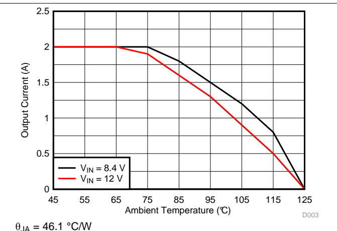
图 19. Thermal Derating, V_{OUT} = 5 \text{ V}
