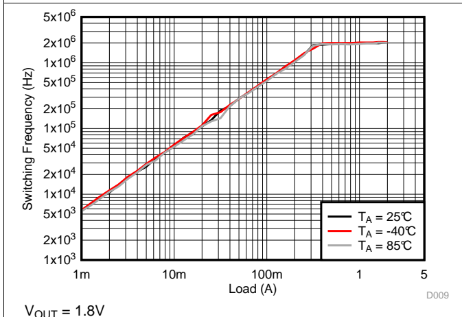
图 22. Switching Frequency
