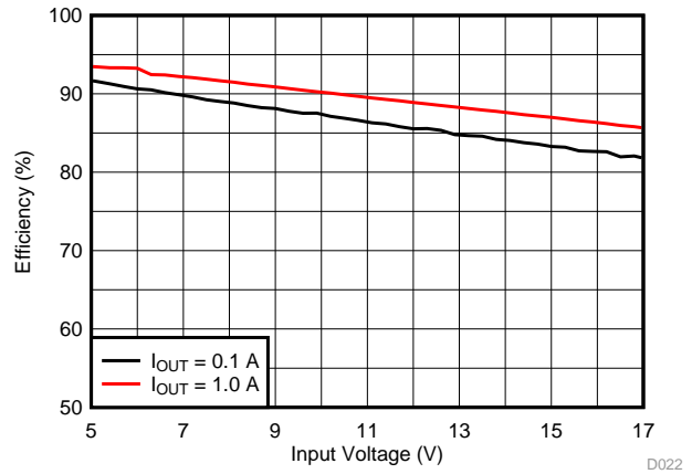
图 13. Efficiency, V_{OUT} = 3.3\text{ V}
