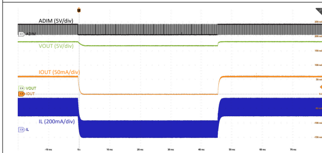
调光占空比 90% → 1% → 90%
