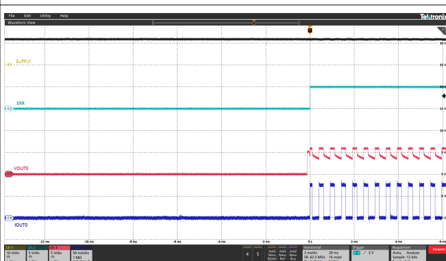
Figure 7-26. LED Open-Circuit Recovery In FS Mode
