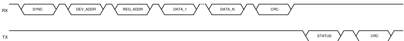
图 6-18. Multiple Data Bytes Write in Burst Mode
