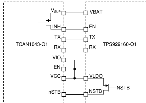
图 6-7. Sleep Mode Typical Application Diagram
