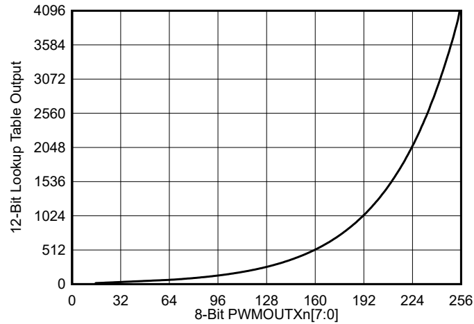
图 6-5. PWM Duty Cycle vs 8-Bit Code for Exponential Dimming
