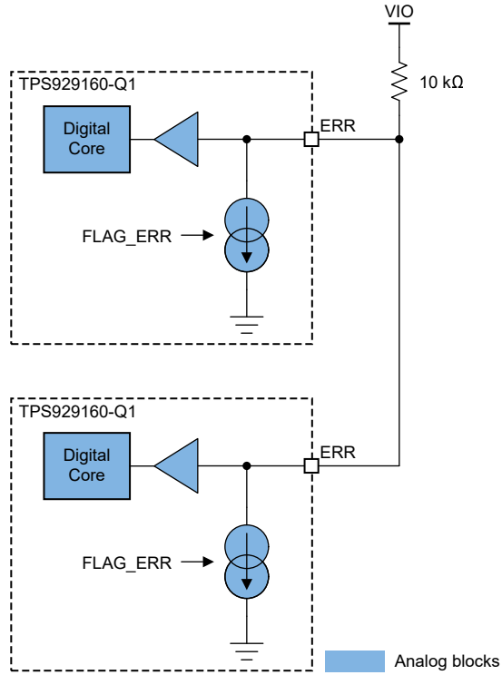
图 6-10. \overline{\text{ERR}} Internal Block Diagram
