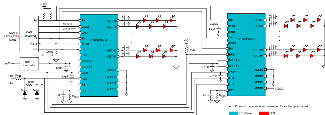
图 7-2. Typical Application Schematic
