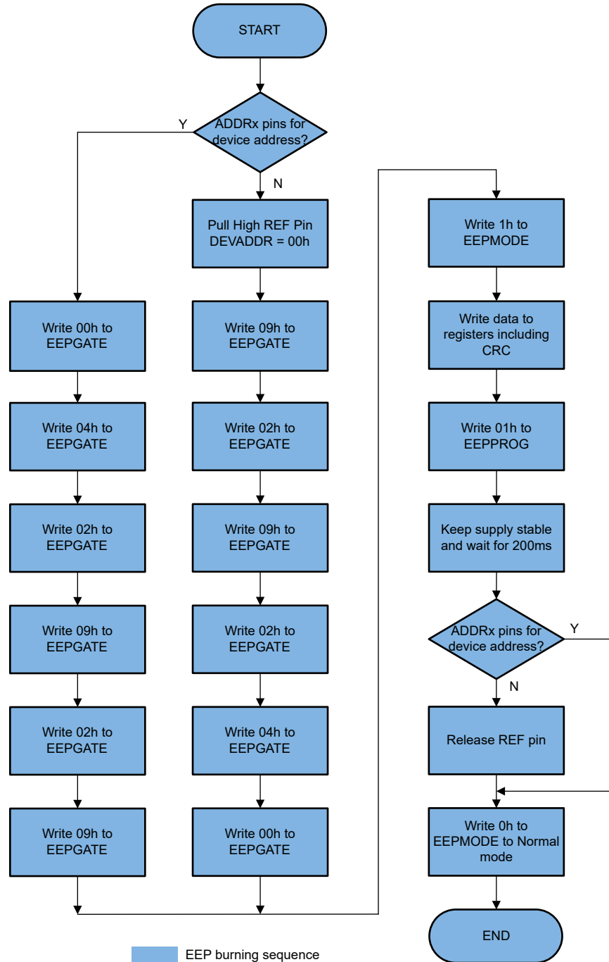
图 6-20. Programming Sequence
