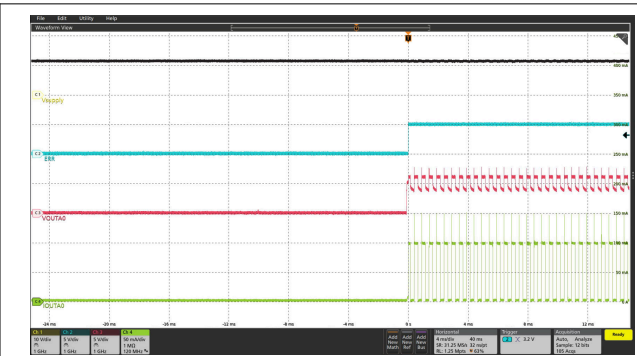
图 5-31. LED Short-Circuit Recovery in Fail-Safe Mode
