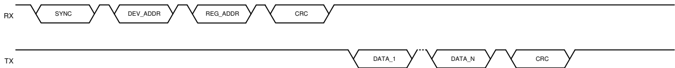
图 6-19. Multiple Data Bytes Read in Burst Mode
