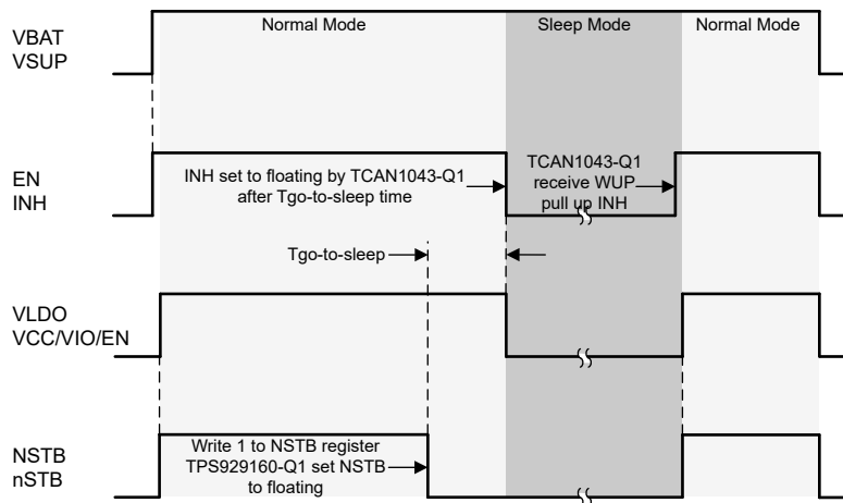
图 6-8. Sleep Mode Access and Exit Timing Diagram
