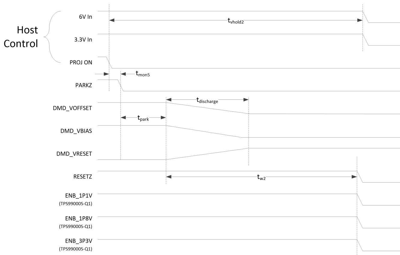
图 5-3. Power Down Timing—PROJ_ON Trigger
