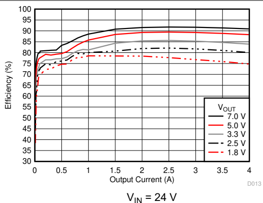
图 6-13. Efficiency versus Output Current
