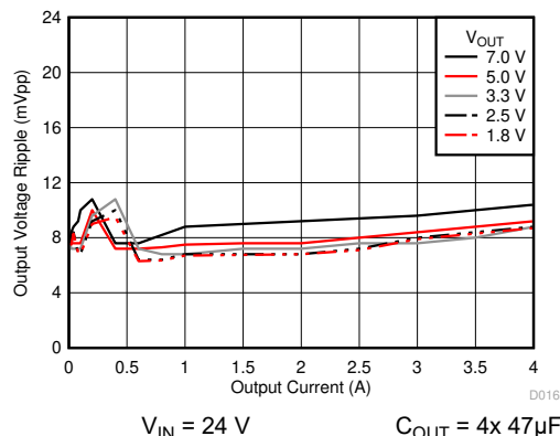
图 6-16. Voltage Ripple versus Output Current
