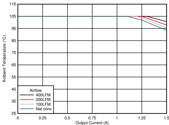
图 7-11. Safe Operating Area (V OUT = 5.0 V)
