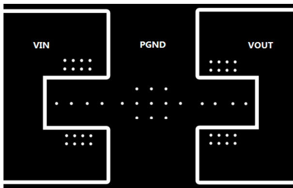
图 11-3. Typical Mid-Layer
