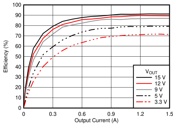
图 7-13. Efficiency
