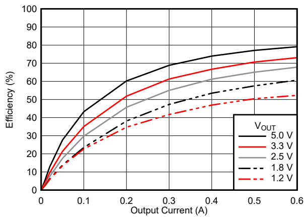
图 6-13. Efficiency
