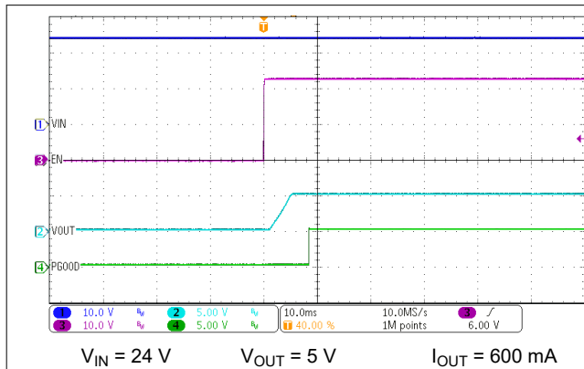
图 8-2. Start-Up Waveforms
