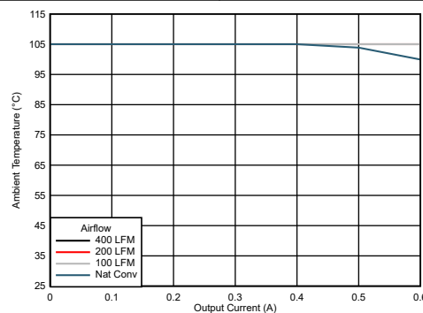
图 6-17. Safe Operating Area ( V_{OUT} = 5.0\text{ V} )
