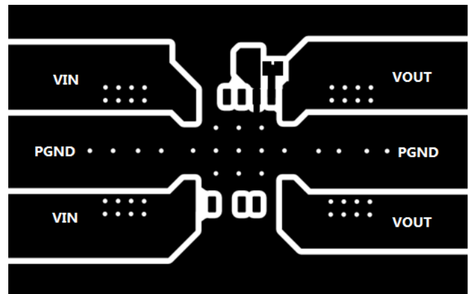
图 10-2. Typical Top-Layer
