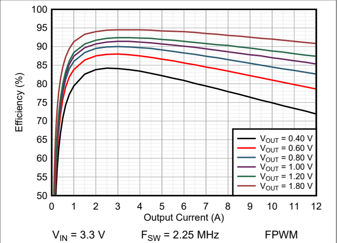
图 9-11. Efficiency TPSM8287A12BBS
