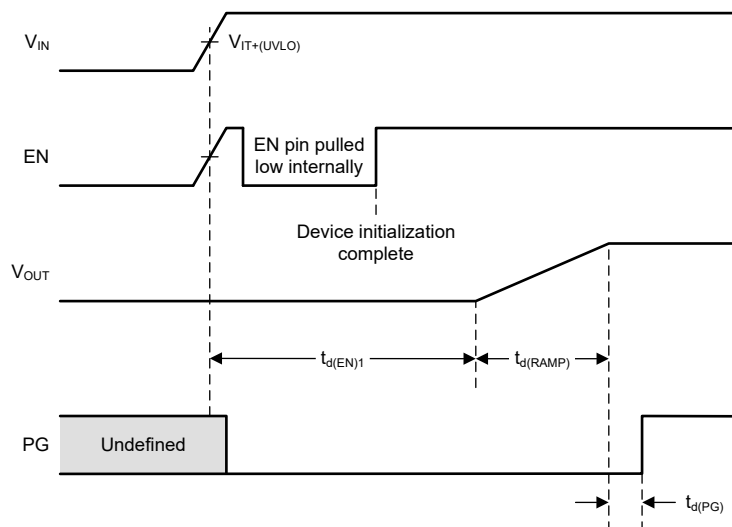
图 7-11. Start-Up Timing When EN is Pulled Up to V IN
