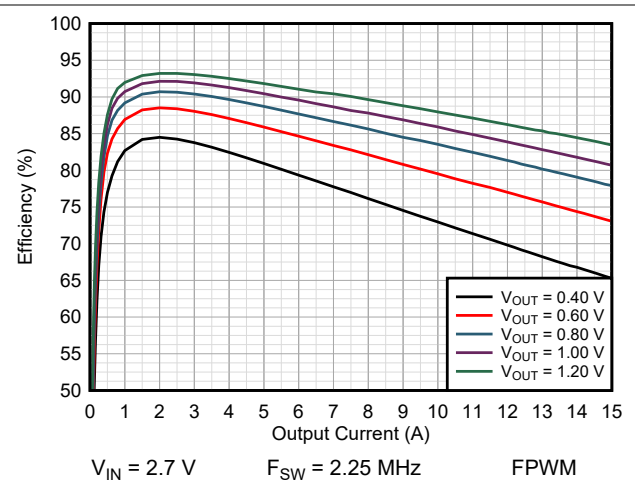
图 9-15. Efficiency TPSM8287A15BBH
