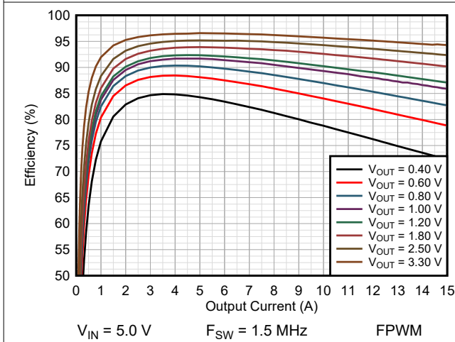
图 9-18. Efficiency TPSM8287A15BAH
