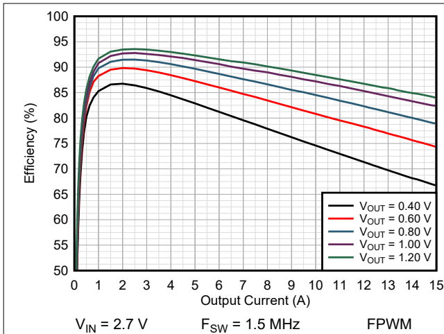
图 9-14. Efficiency TPSM8287A15BAH
