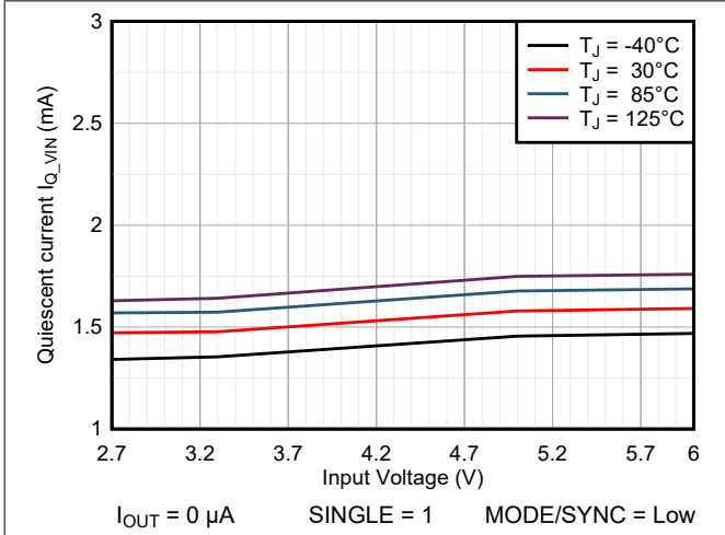
图 6-1. Operating Supply Current (Power-Save Mode)
