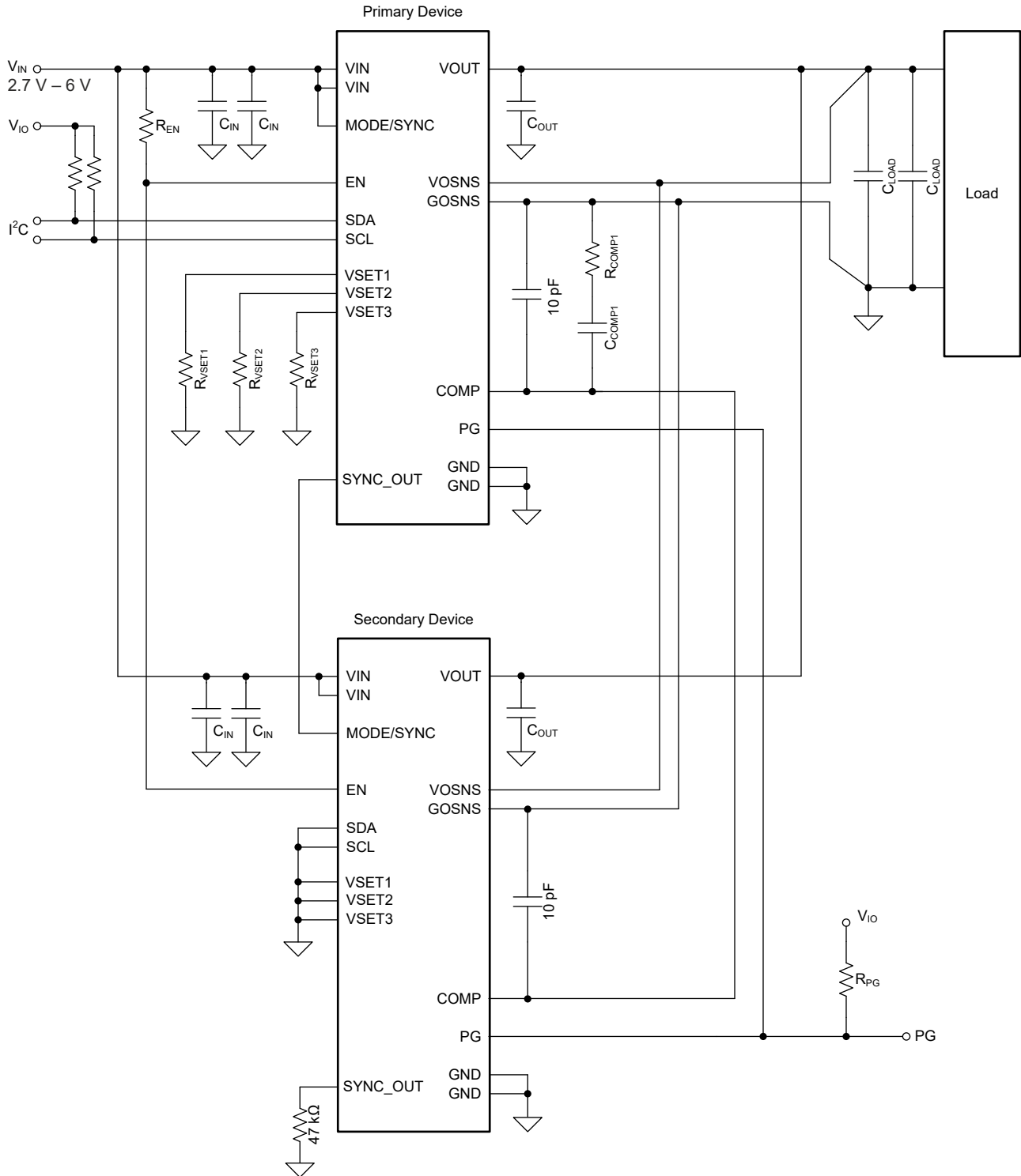
图 7-22. Two TPSM8287Axx Devices in a Stacked Configuration
