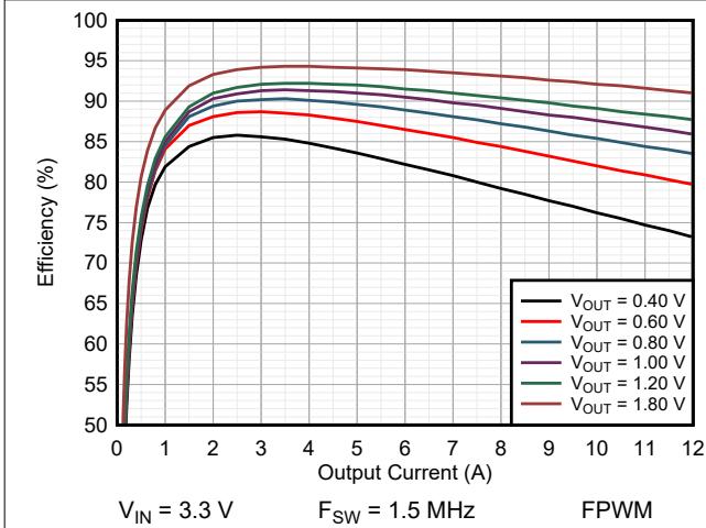
图 9-10. Efficiency TPSM8287A12BAS
