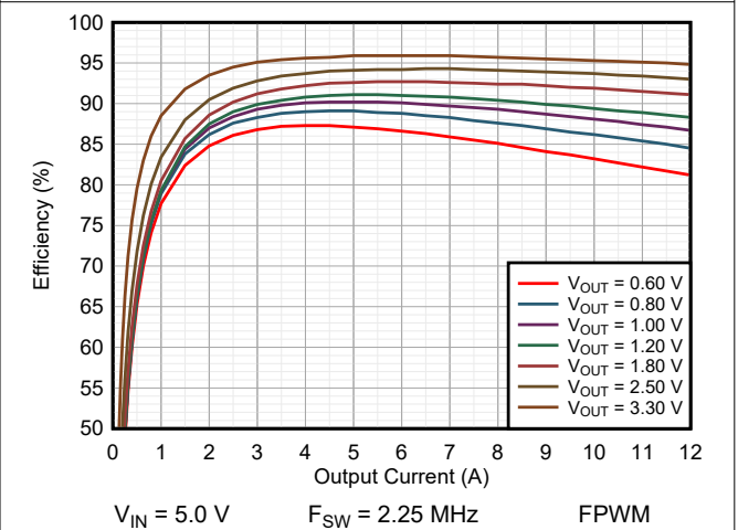
图 9-13. Efficiency TPSM8287A12BBS
