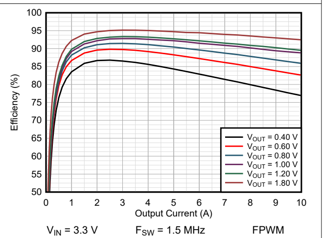
图 9-5. Efficiency TPSM8287A10BAH
