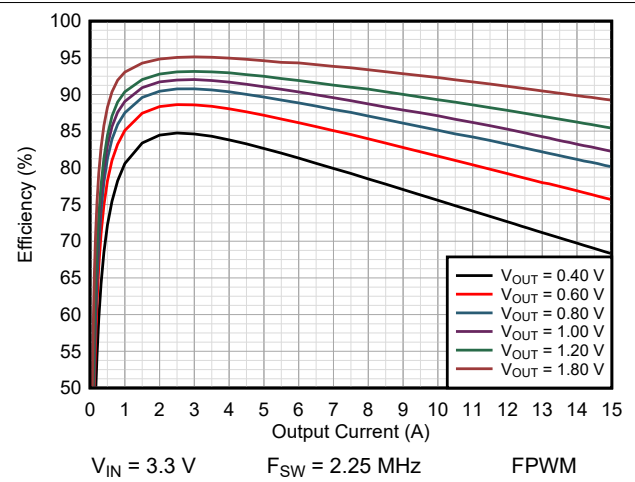
图 9-17. Efficiency TPSM8287A15BBH
