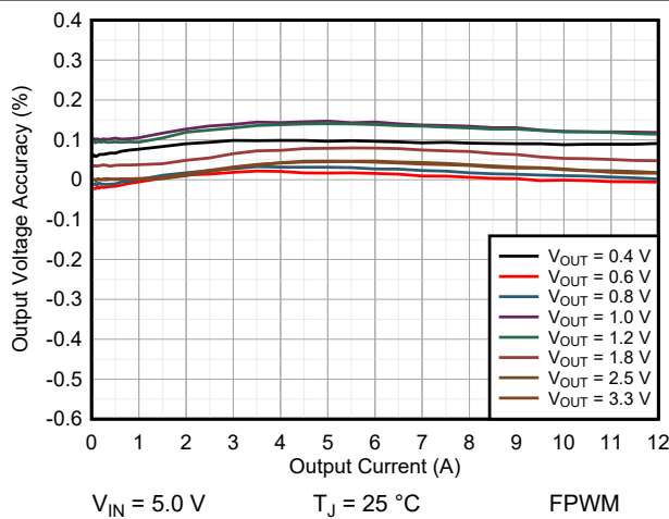
图 9-24. Load Regulation TPSM8287A12BAS
