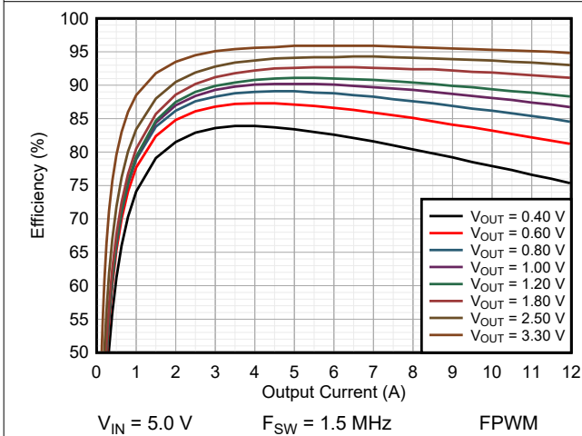
图 9-12. Efficiency TPSM8287A12BAS
