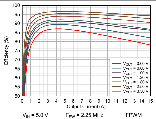
图 9-19. Efficiency TPSM8287A15BBH
