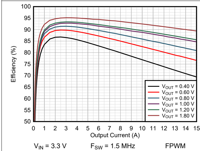
图 9-16. Efficiency TPSM8287A15BAH
