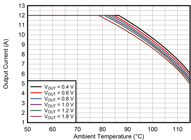
图 9-40. Safe Operating Area TPSM8287A10BAH V_{IN} = 3.3\text{ V}
