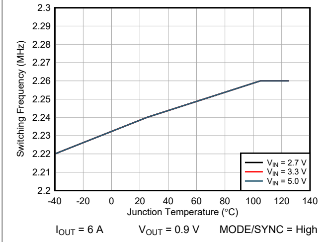
图 6-3. TPSM8287A12BBS Switching Frequency vs T J
