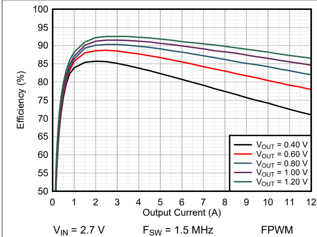
图 9-8. Efficiency TPSM8287A12BAS
