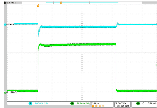
V_{IN} = 12\text{ V} I_O = 5\text{ mA to } 1\text{ A to } 5\text{ mA} V_{OUT} = 3.3\text{ V} 2.5-MHz Auto PFM/PWM T_A = 25^\circ\text{C}
