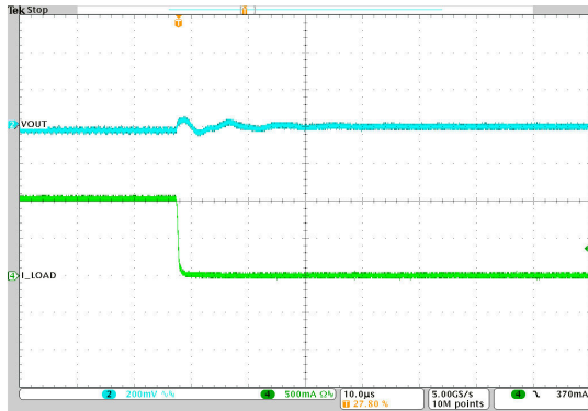
V_{IN} = 12\text{ V} 1-MHz Auto PFM/PWM I_O = 1\text{ A to } 5\text{ mA} V_{OUT} = 1.2\text{ V} T_A = 25^\circ\text{C}
