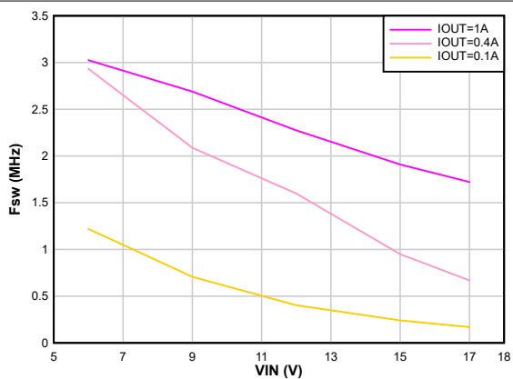
8-21. Switching Frequency vs Input Voltage V_{OUT} = 3.3\text{ V} Auto PFM/PWM F_{sw} = 2.5\text{ MHz}
