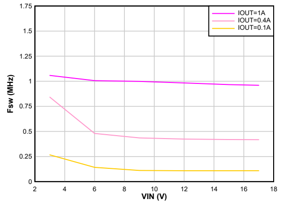
8-18. Switching Frequency vs Input Voltage V_{OUT} = 1.8\text{ V} Auto PFM/PWM F_{sw} = 1\text{ MHz}
