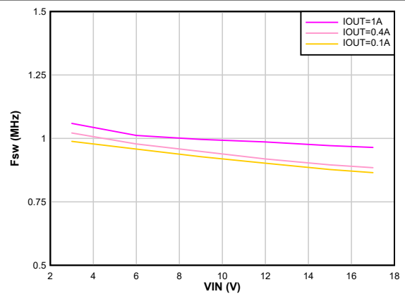
8-20. Switching Frequency vs Input Voltage V_{OUT} = 1.8\text{ V} FPWM F_{sw} = 1\text{ MHz}
