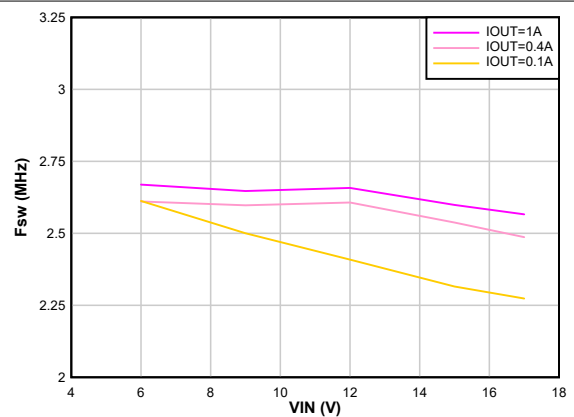
8-22. Switching Frequency vs Input Voltage V_{OUT} = 3.3\text{ V} FPWM F_{sw} = 2.5\text{ MHz}
