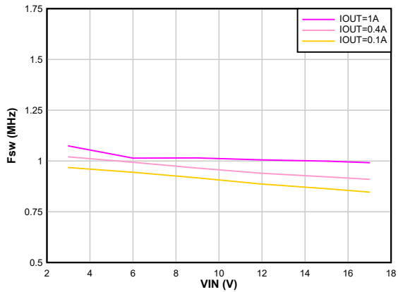
8-17. Switching Frequency vs Input Voltage V_{OUT} = 1.2\text{ V} FPWM F_{sw} = 1\text{ MHz}
