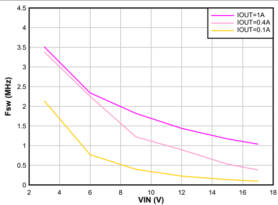
8-19. Switching Frequency vs Input Voltage V_{OUT} = 1.8\text{ V} Auto PFM/PWM F_{sw} = 2.5\text{ MHz}
