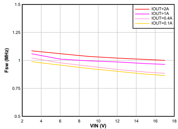
8-20. Switching Frequency vs Input Voltage V_{OUT} = 1.2\text{ V} FPWM F_{sw} = 1\text{ MHz}
