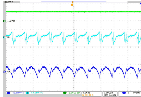
V_{IN} = 12\text{ V} 1-MHz Auto I_O = 2\text{ A} PFM/PWM V_{OUT} = 1.2\text{ V} T_A = 25^\circ\text{C}
