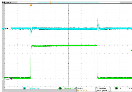
V_{IN} = 12\text{ V} 2.5-MHz FPFM I_O = 5\text{ mA to } 2\text{ A to } 5\text{ mA} V_{OUT} = 3.3\text{ V} T_A = 25^\circ\text{C}
