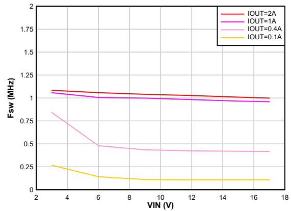
8-18. Switching Frequency vs Input Voltage V_{OUT} = 1.8\text{ V} Auto PFM/PWM F_{sw} = 1\text{ MHz}
