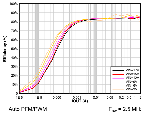
图 8-9. Efficiency vs Output Current V_{OUT} = 1.8 \text{ V}
