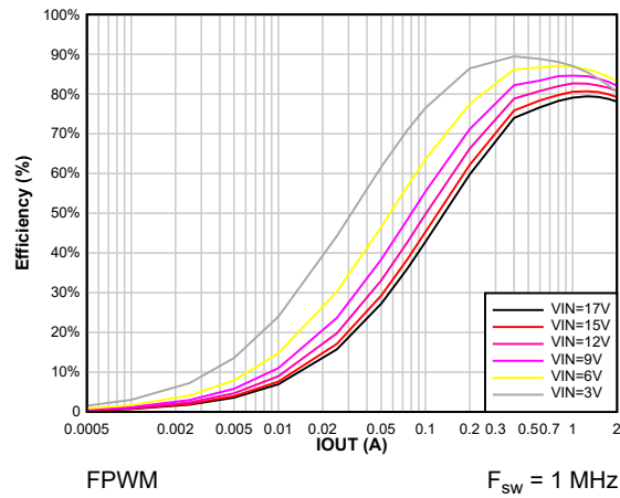
图 8-7. Efficiency vs Output Current V_{OUT} = 1.2 \text{ V}
