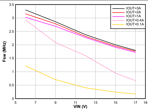
Auto PFM/PWM F_{sw} = 2.5 \text{ MHz} 8-21. Switching Frequency vs Input Voltage V_{OUT} = 3.3 \text{ V}
