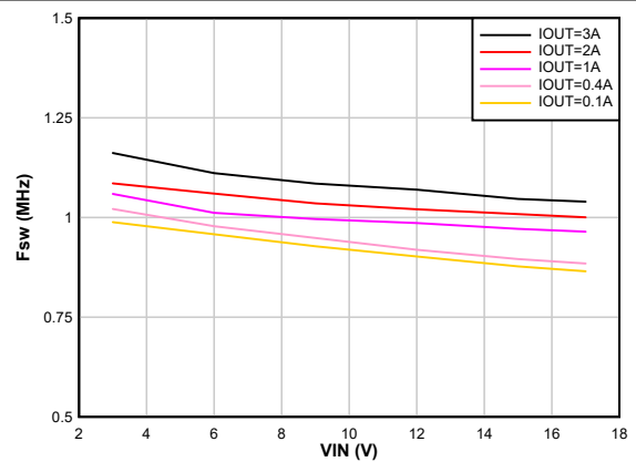
FPWM F_{sw} = 1 \text{ MHz} 8-20. Switching Frequency vs Input Voltage V_{OUT} = 1.8 \text{ V}
