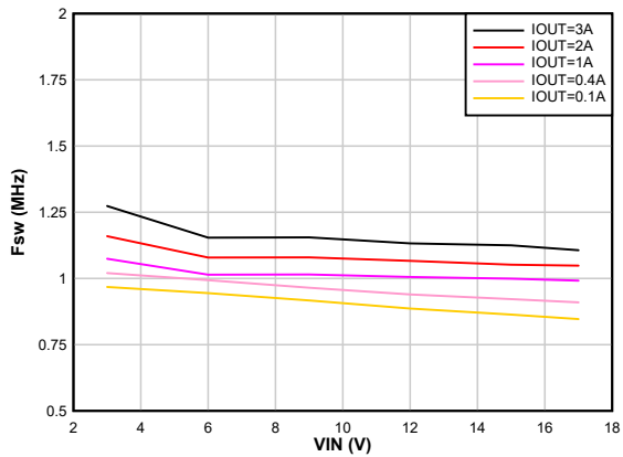
FPWM F_{sw} = 1 \text{ MHz} 8-17. Switching Frequency vs Input Voltage V_{OUT} = 1.2 \text{ V}
