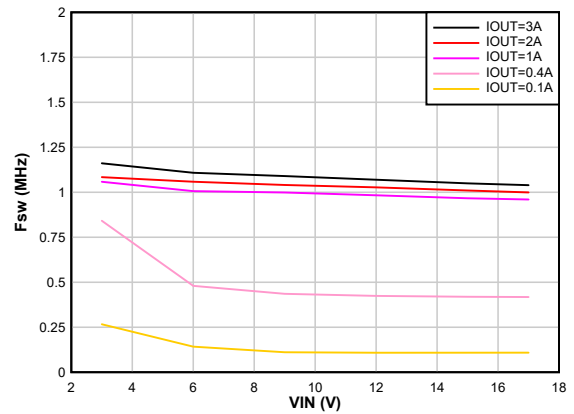
Auto PFM/PWM F_{sw} = 1 \text{ MHz} 8-18. Switching Frequency vs Input Voltage V_{OUT} = 1.8 \text{ V}
