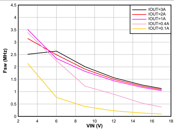
Auto PFM/PWM F_{sw} = 2.5 \text{ MHz} 8-19. Switching Frequency vs Input Voltage V_{OUT} = 1.8 \text{ V}
