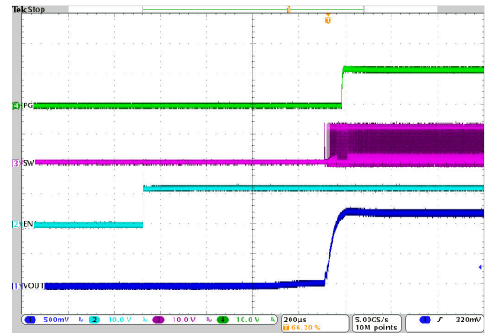
V_{IN} = 12 \text{ V} 1\text{-MHz FPWM} I_O = 0 \text{ mA} V_{OUT} = 1.2 \text{ V} T_A = 25^\circ\text{C}
