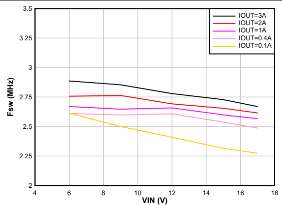
FPWM F_{sw} = 2.5 \text{ MHz} 8-22. Switching Frequency vs Input Voltage V_{OUT} = 3.3 \text{ V}
