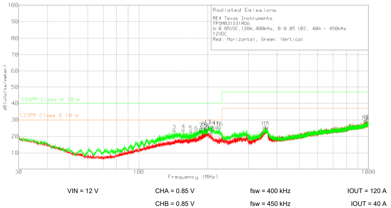
图 8-15. Radiated EMI
