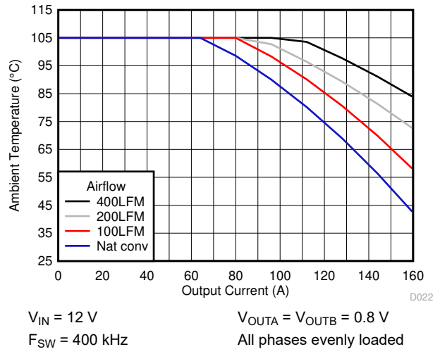
图 6-8. Thermal Safe Operating Area
