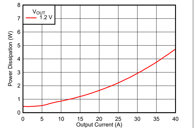
图 8-5. VOUTB Power Dissipation
