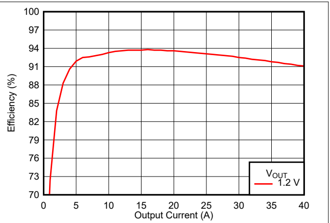
图 8-3. VOUTB Efficiency
