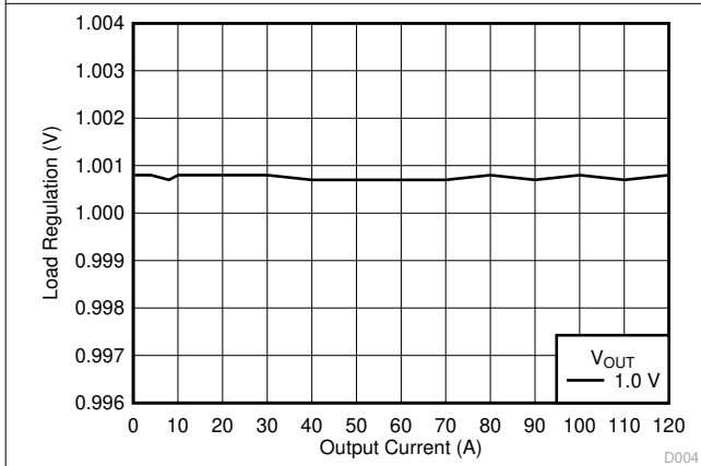
图 6-5. VOUTA Load Regulation
