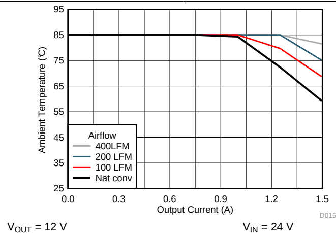
图 15. Safe Operating Area
